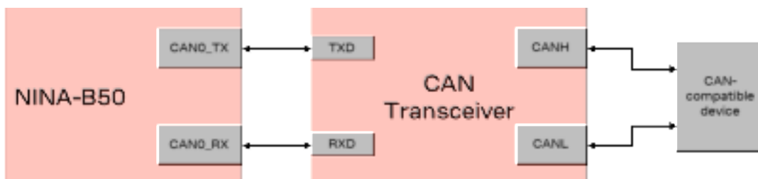
Figure 7: FlexCAN implementation
