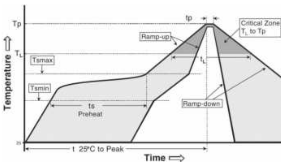
Figure 20: Reflow profile
