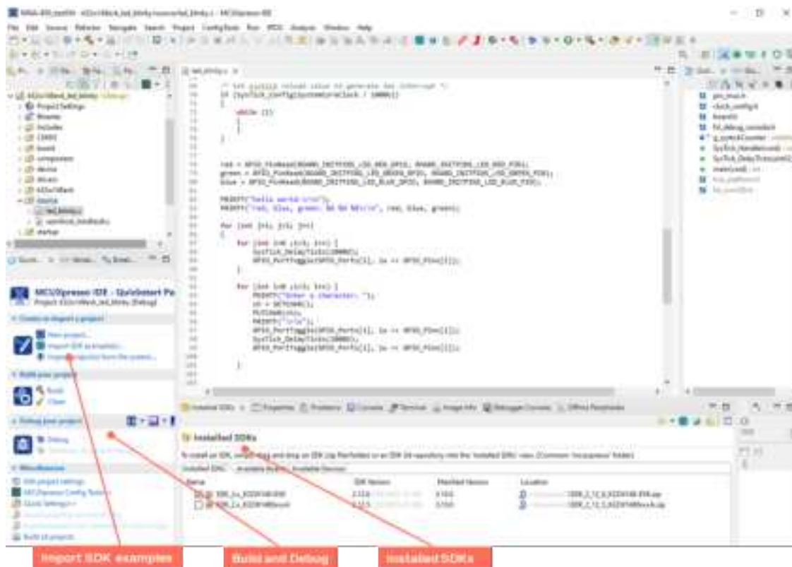
Figure 15: Installed SDKs
