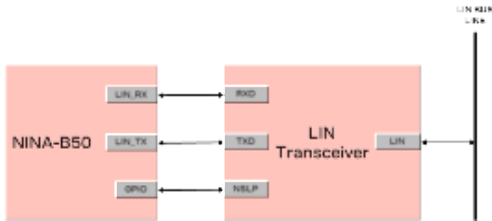
Figure 8: LIN implementation
