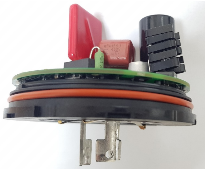
Platform (NEMA3) card-on NEMA connector
