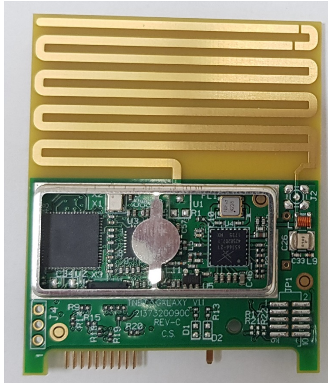
RF Card (TNET3) shield removed- top view
