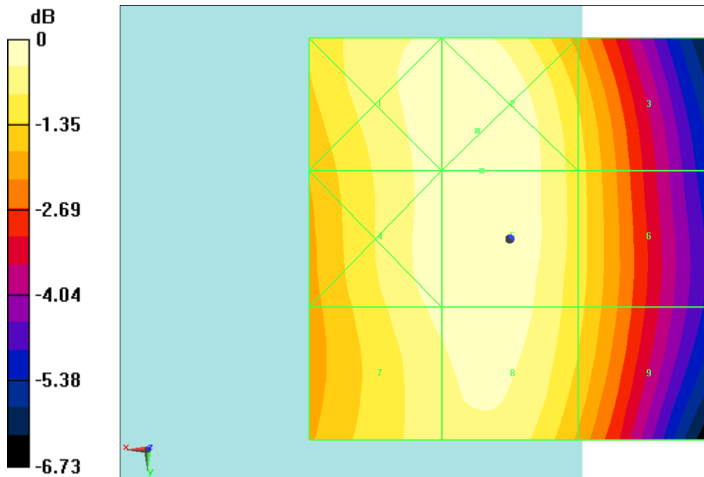
Fig B.2 HAC RF E-Field GSM 850 Middle
