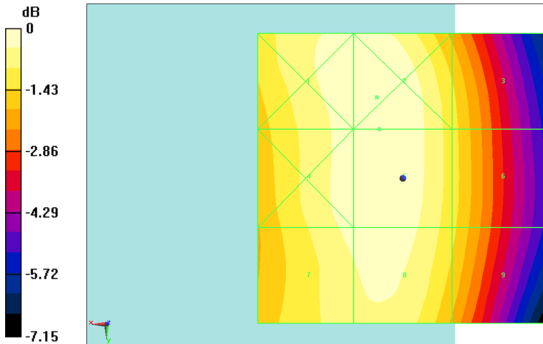
Fig B.1 HAC RF E-Field GSM 850 High
