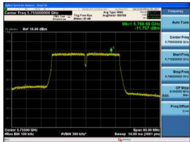
Channel 151 (5755MHz)
