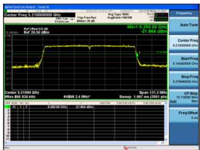
802.11ac-VHT80 - Channel 42 (5210MHz)
