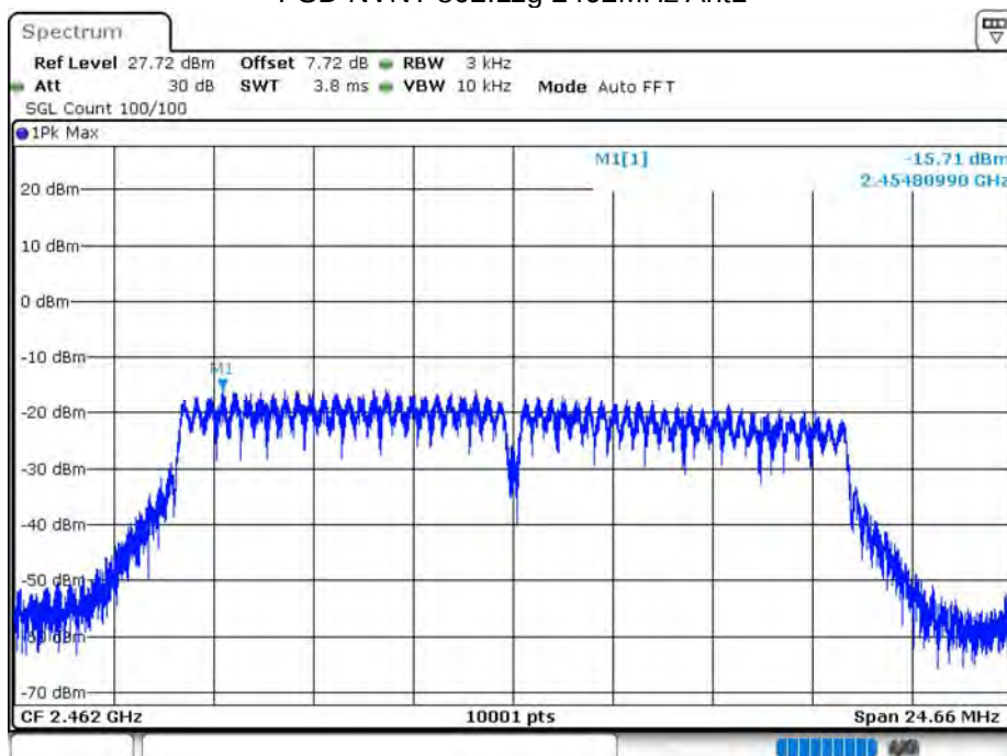
PSD NVNT 802.11g 2462MHz Ant1
