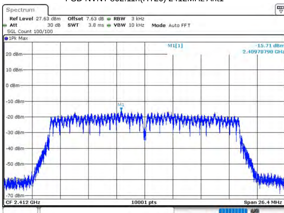
PSD NVNT 802.11n(HT20) 2412MHz Ant1
