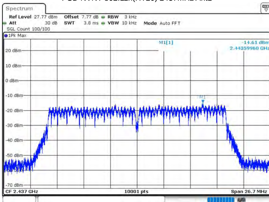
PSD NVNT 802.11n(HT20) 2437MHz Ant1
