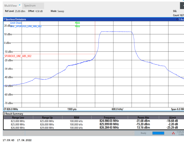
Band5-1.4MHz-QPSK-20427-6RB#0
