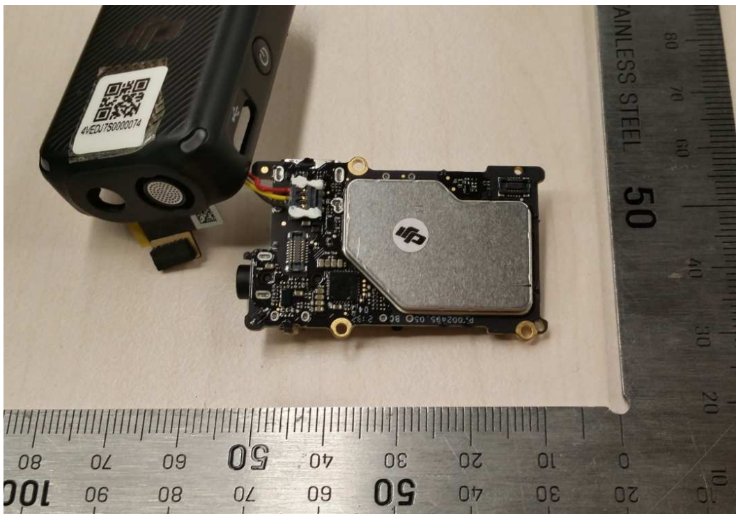
Figure 2: Internal view -2
