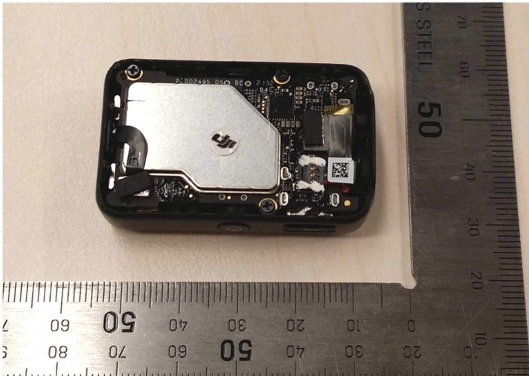
Figure 1: Internal view -1
