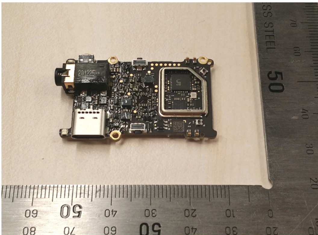
Figure 6: Mainboard view -2
