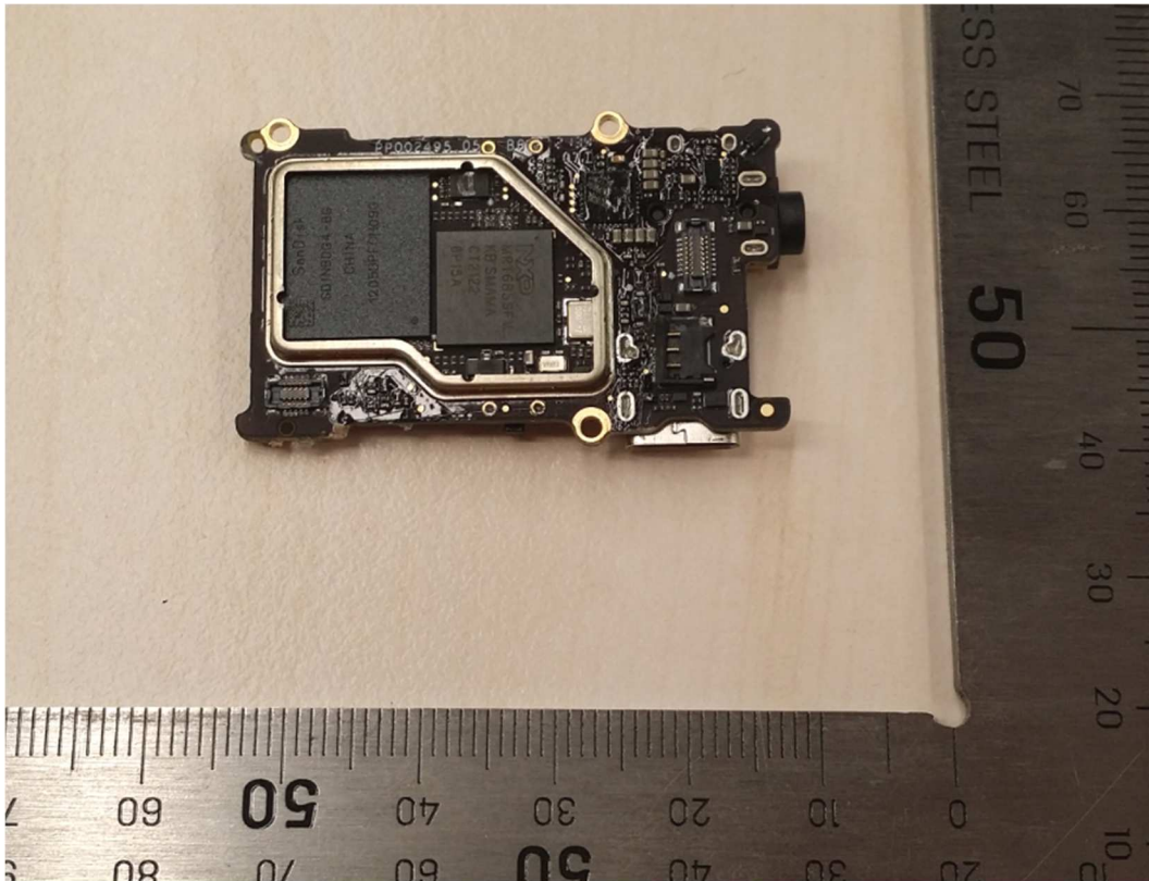
Figure 5: Mainboard view -1
