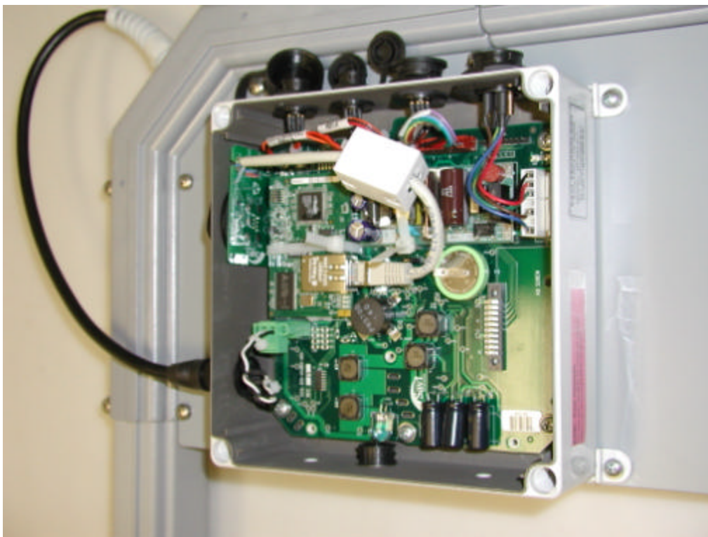
Device with external antenna
