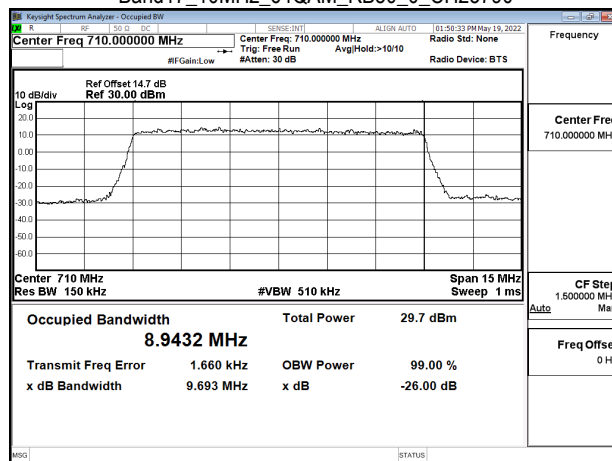
Band17_10MHz_64QAM_RB50_0_CH23800
