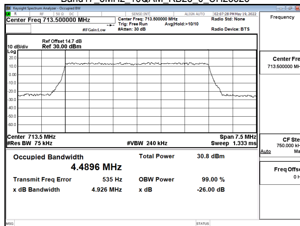
Band17_5MHz_16QAM_RB25_0_CH23825
