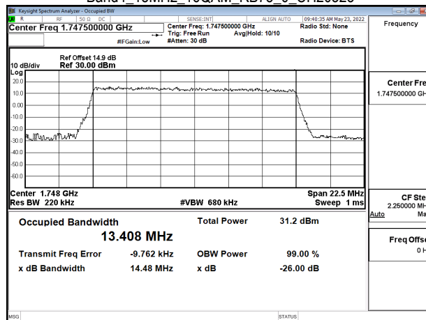
Band4_15MHz_16QAM_RB75_0_CH20325
