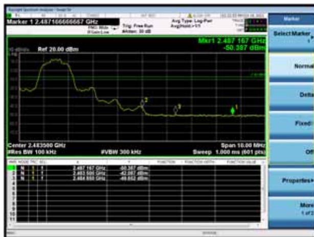
8-DPSK HIGH CHANNEL, BAND EDGE
