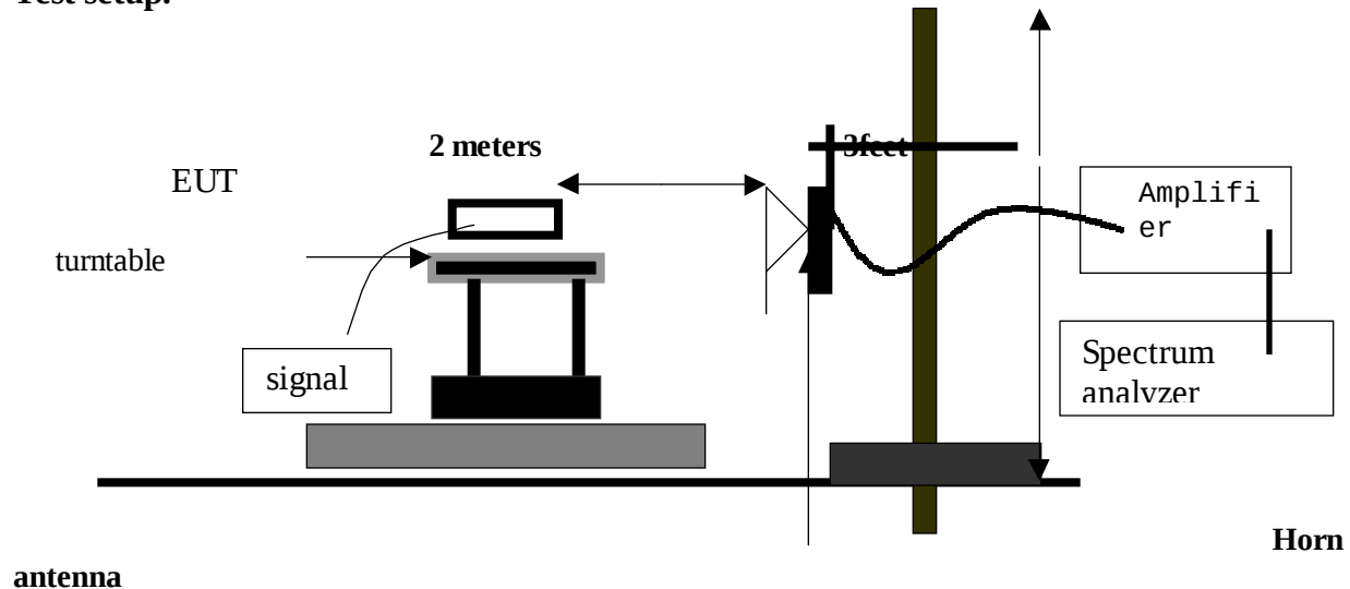
Radiated Emissions Configuration
