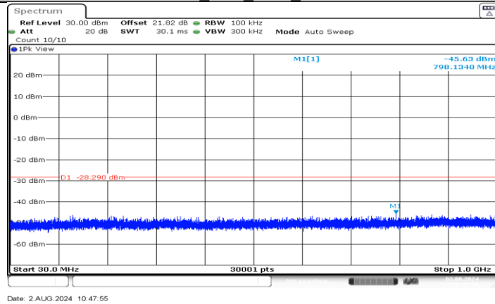
11N40SISO_Ant2_2452_30-1000
