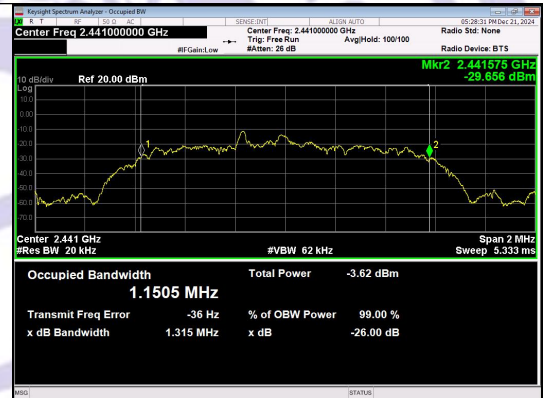
8DPSK_3-DH1_Channel 39
