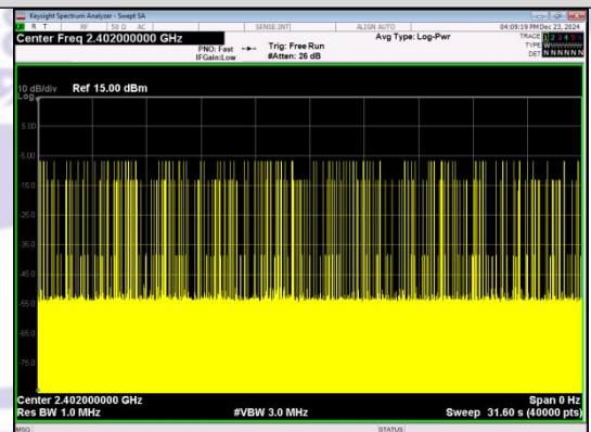
Number of Pulses in 31.6 seconds n/4DQPSK_2-DH5
