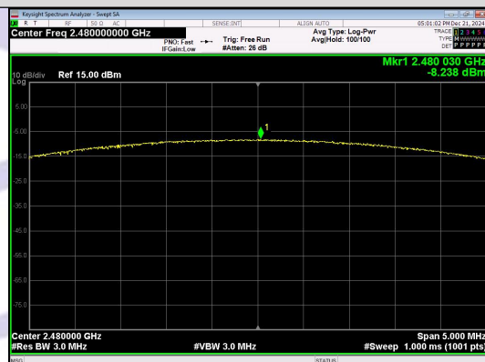
Peak Output Power n/4DQPSK_Channel 78
