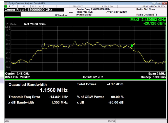
n/4QPSK_2-DH1_Channel 78
