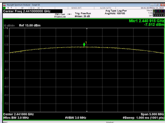
Peak Output Power n/4DQPSK_Channel 39
