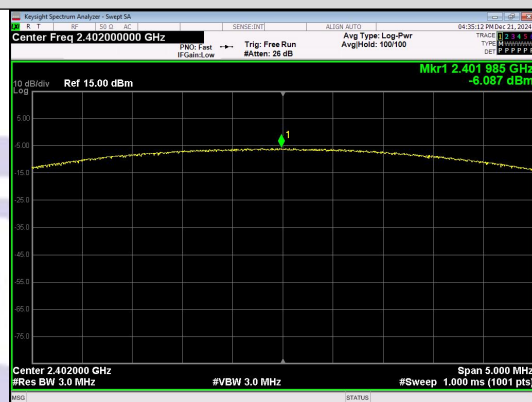
Peak Output Power n/4DQPSK_Channel 0
