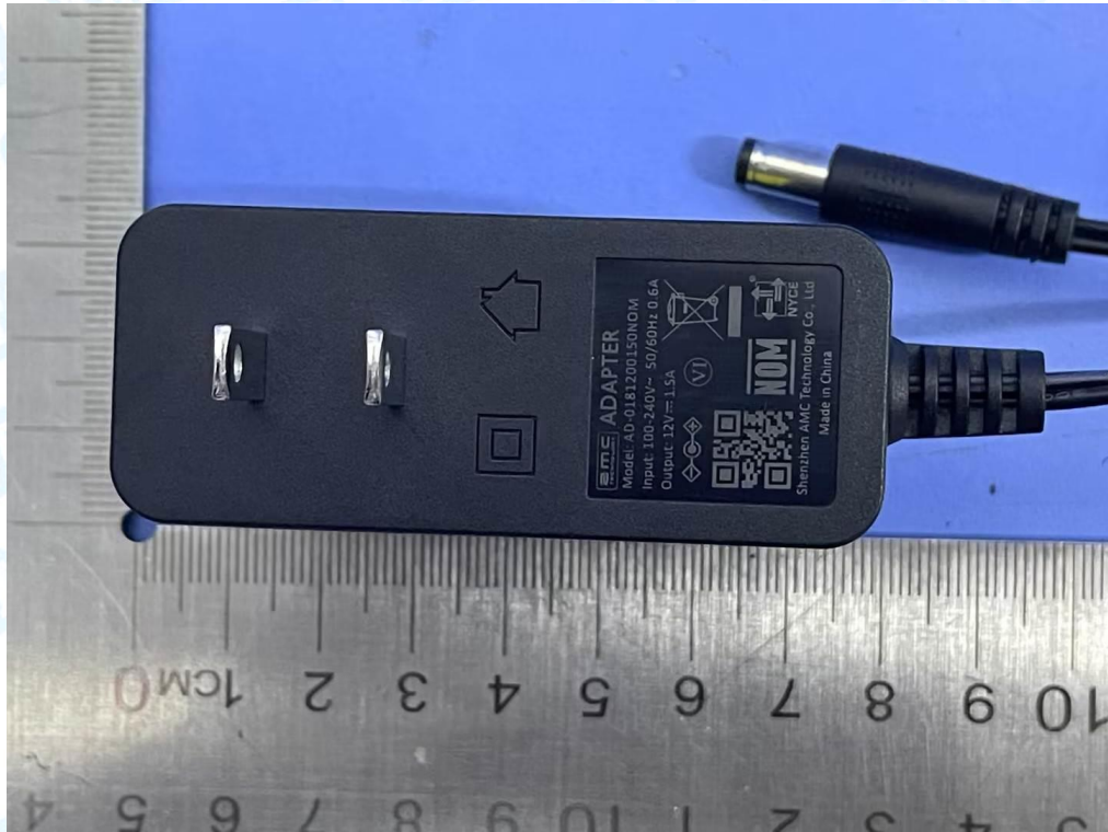
Photo 8 Appearance of Adapter-NP3081GB
