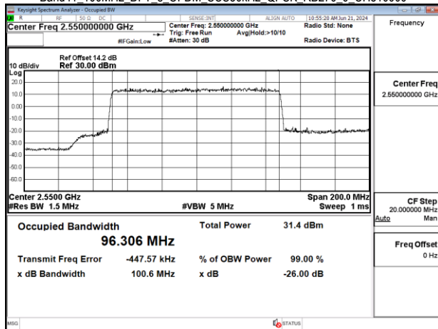
Band41_100MHz_DFT_s_OFDM_SCS30kHz_QPSK_RB270_0_CH518598
