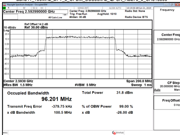
Band41_100MHz_DFT_s_OFDM_SCS30kHz_QPSK_RB270_0_CH518598
