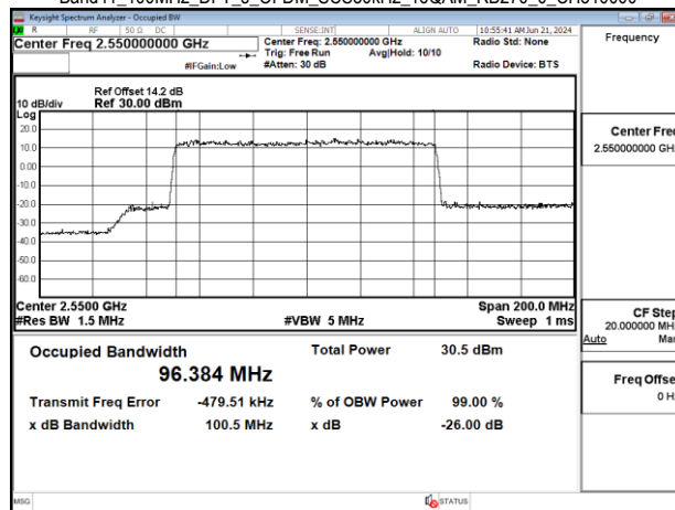
Band41_100MHz_DFT_s_OFDM_SCS30kHz_16QAM_RB270_0_CH510000
