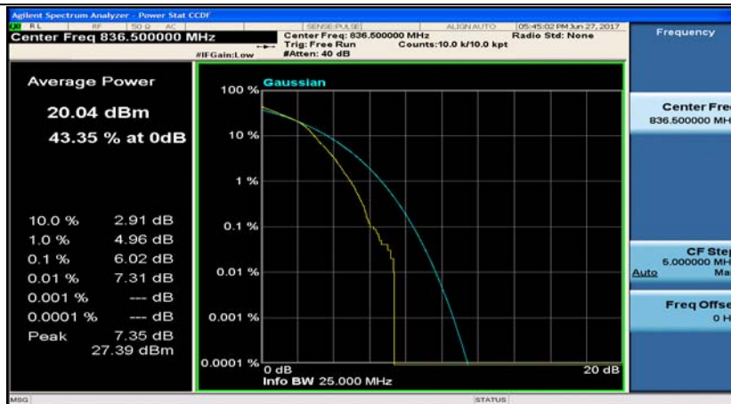
Band5_5MHz_QPSK_20525_25RB#0
