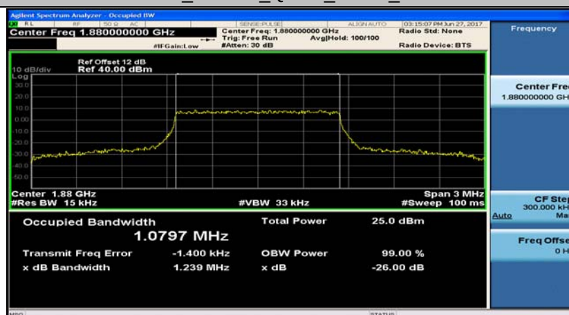
Band2_1.4MHz_16QAM_18900_6RB#0
