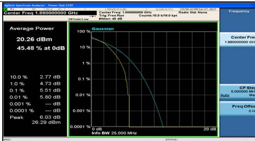
Band2_20MHz_QPSK_18900_100RB#0
