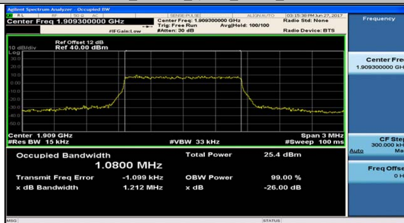
Band2_1.4MHz_16QAM_19193_6RB#0
