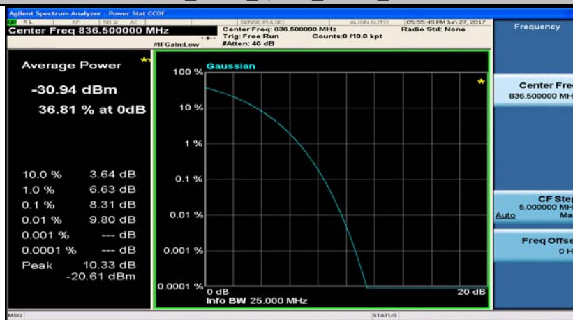
Band5_5MHz_16QAM_20525_25RB#0
