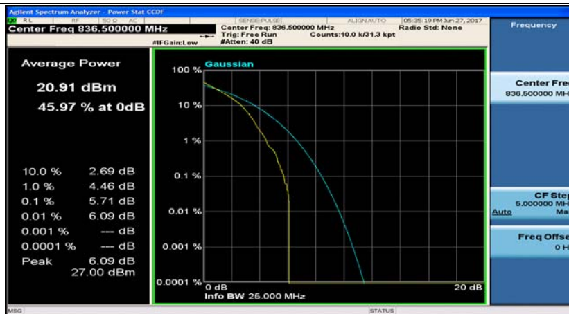
Band5_1.4MHz_16QAM_20525_6RB#0
