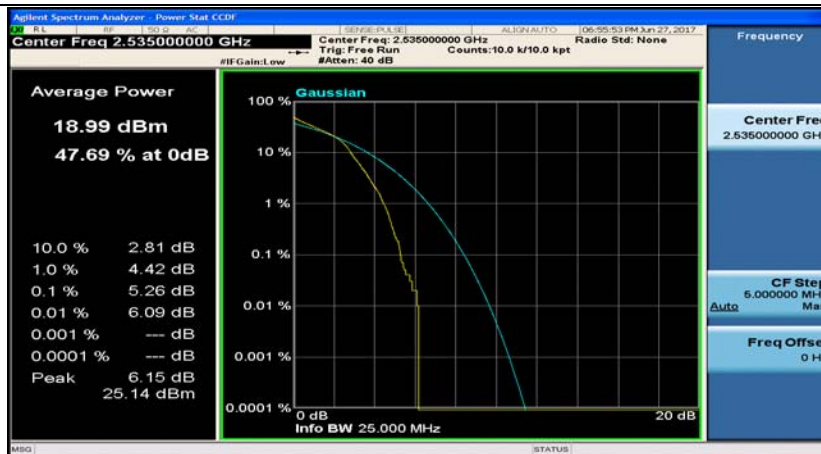
Band7_10MHz_QPSK_21100_50RB#0
