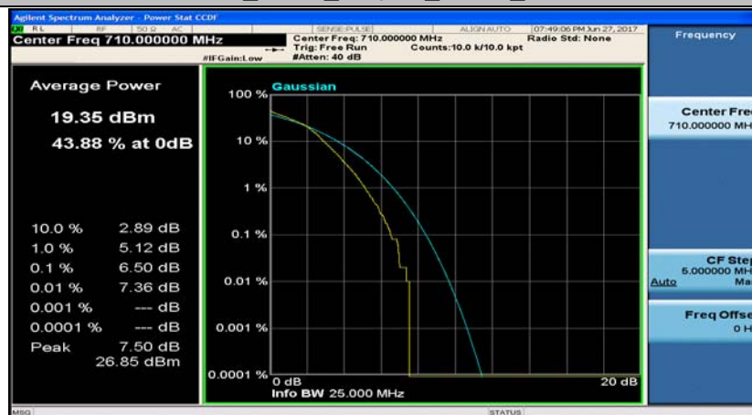
Band17_10MHz_QPSK_23790_50RB#0
