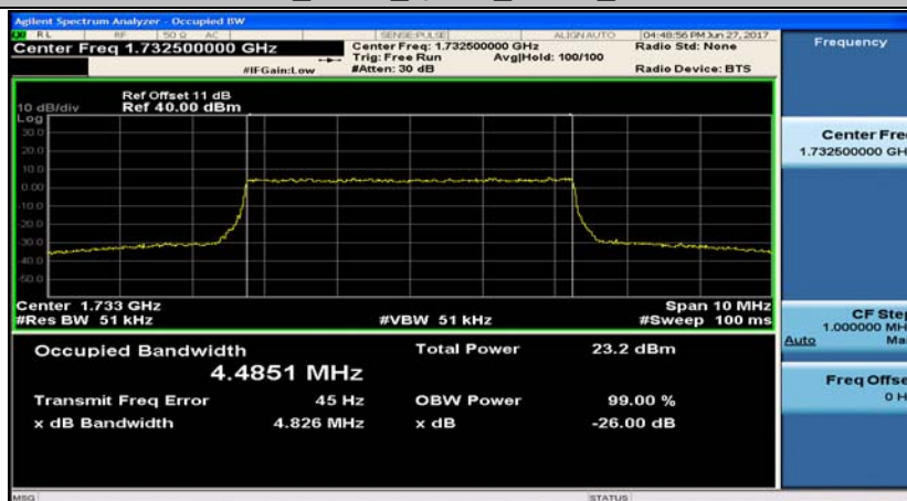
Band4_5MHz_16QAM_20175_25RB#0
