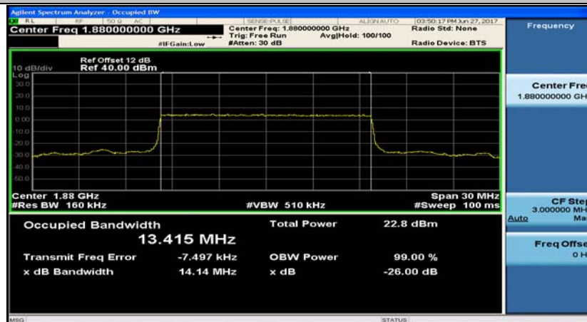
Band2_15MHz_16QAM_18900_75RB#0
