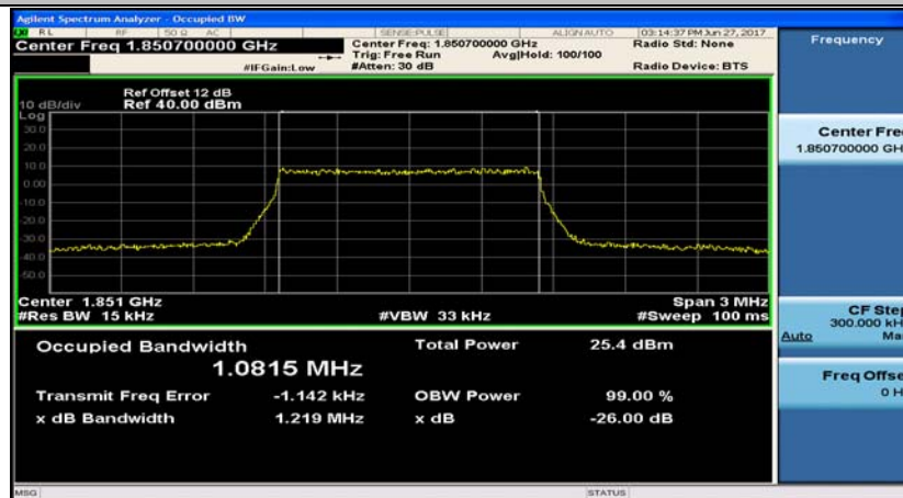
Band2_1.4MHz_16QAM_18607_6RB#0
