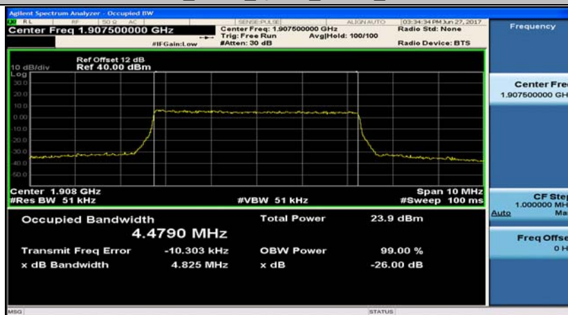
Band2_5MHz_16QAM_19175_25RB#0
