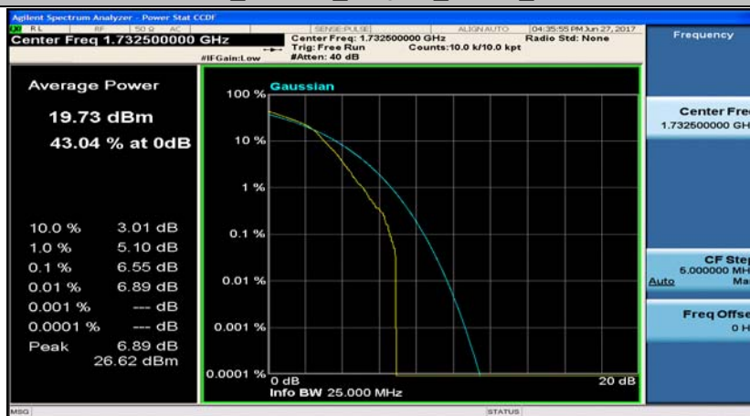
Band4_3MHz_QPSK_20175_15RB#0
