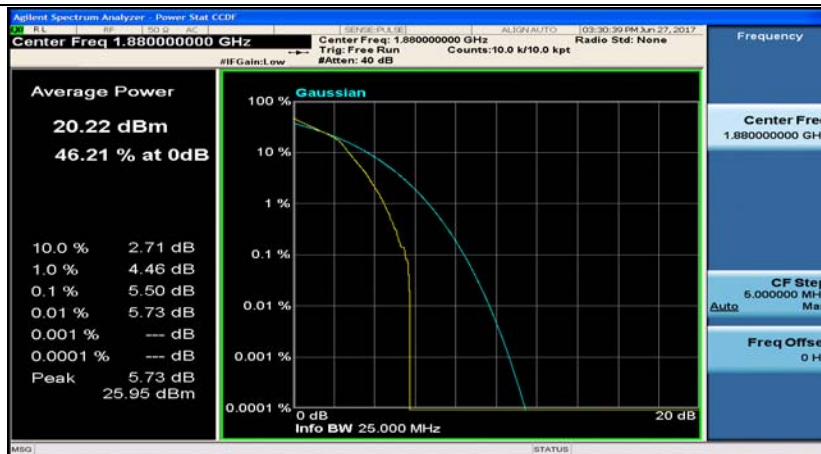
Band2_5MHz_QPSK_18900_25RB#0
