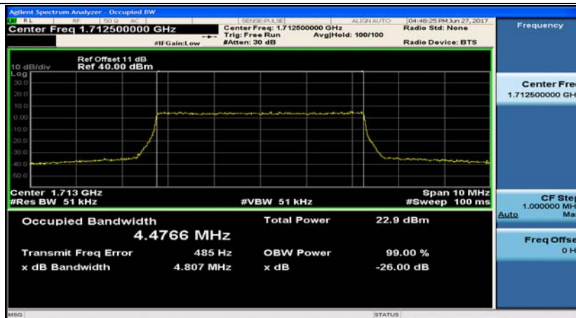
Band4_5MHz_16QAM_19975_25RB#0
