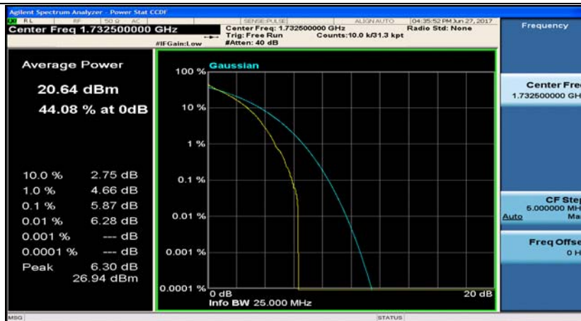
Band4_1.4MHz_16QAM_20175_6RB#0
