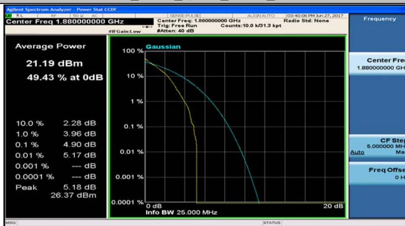
Band2_5MHz_16QAM_18900_25RB#0
