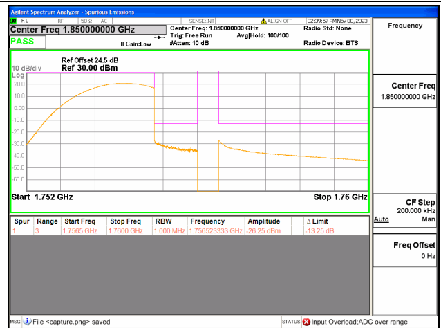
B4 / 1.4MHz / High CH / QPSK / FULL RB
