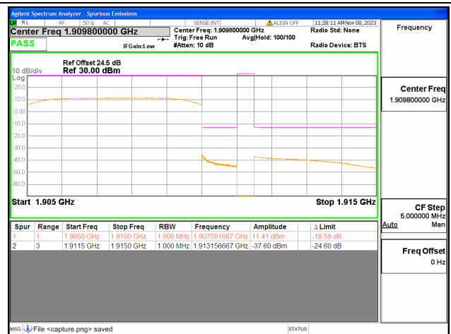
B2 / 5MHz / High CH / QPSK / FULL RB
