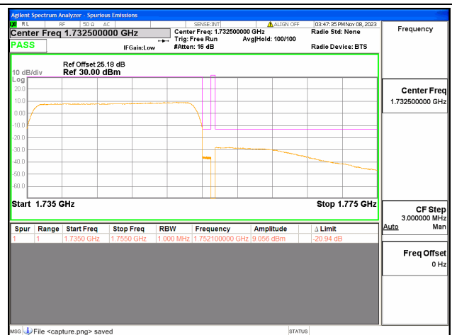
B4 / 20MHz / High CH / QPSK / FULL RB
