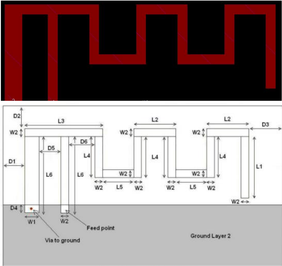
Figure 3: Antenna Dimensions
