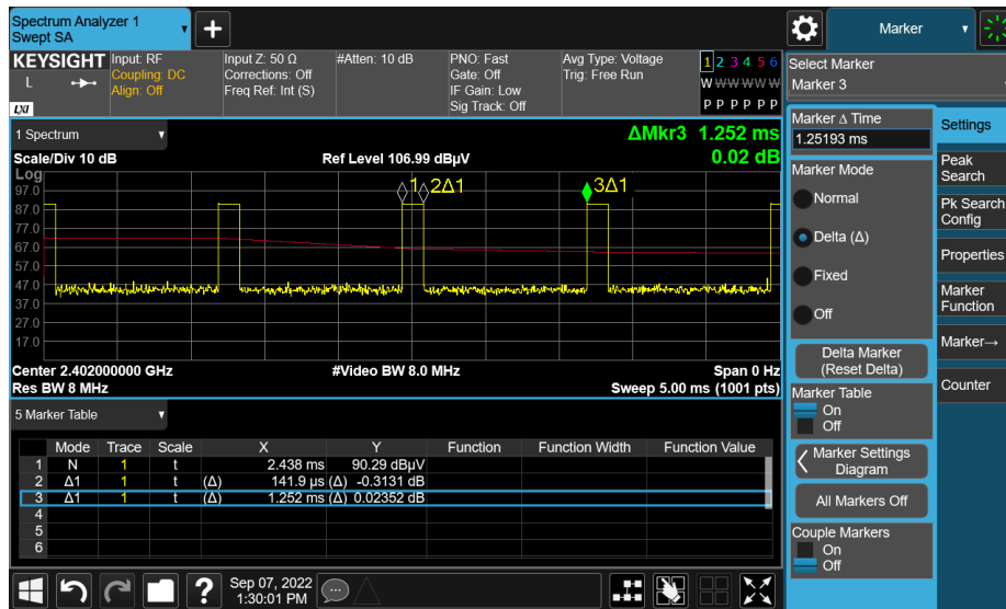
Bluetooth LE 1Mbps Duty Cycle Plot
