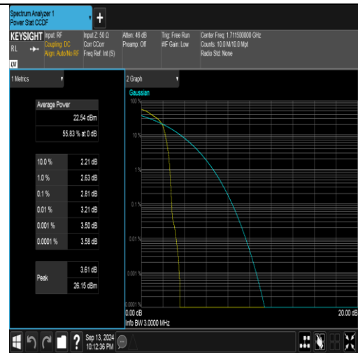
Band66-3MHz-16QAM-131987-1RB#0-PASS
