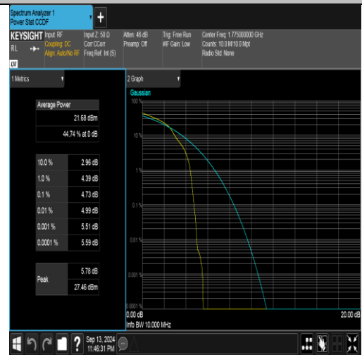
Band66-10MHz-16QAM-132622-1RB#0-PASS
