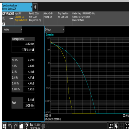
Band66-20MHz-QPSK-132322-1RB#0-PASS
