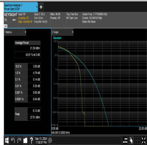
Band66-5MHz-16QAM-132647-1RB#0-PASS
