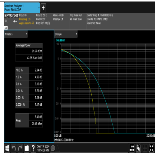
Band66-3MHz-16QAM-132322-15RB#0-PASS
