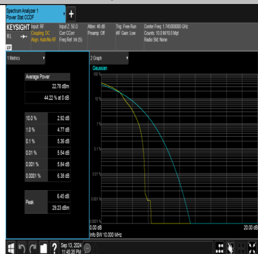
Band66-10MHz-16QAM-132322-1RB#0-PASS
