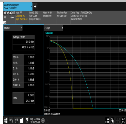
Band66-20MHz-16QAM-132072-100RB#0-PASS
