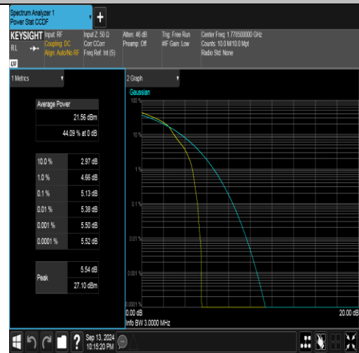
Band66-3MHz-16QAM-132657-1RB#0-PASS
