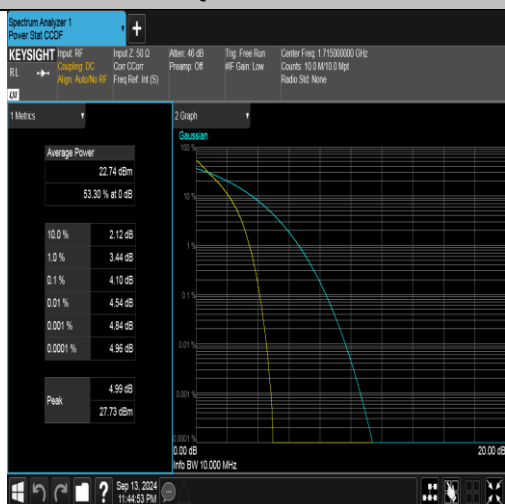
Band66-10MHz-QPSK-132022-50RB#0-PASS
