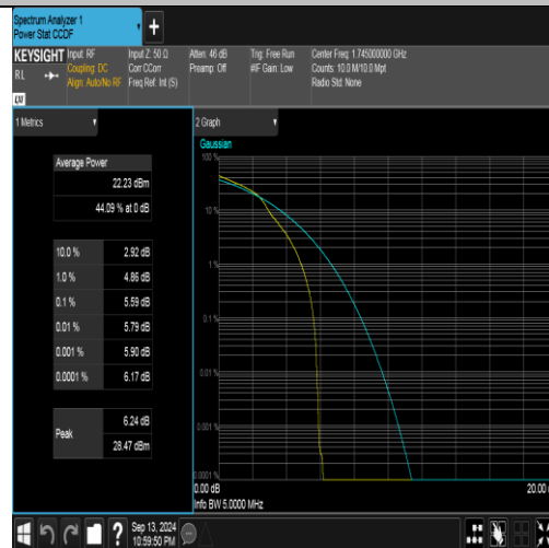
Band66-5MHz-16QAM-132322-1RB#0-PASS
