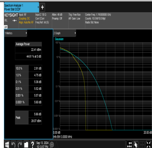
Band66-3MHz-16QAM-132322-1RB#0-PASS
