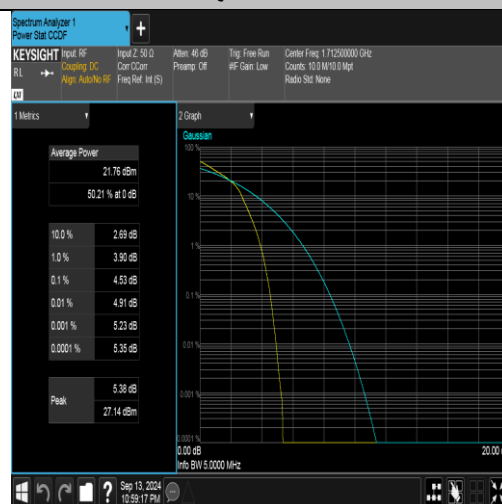
Band66-5MHz-16QAM-131997-25RB#0-PASS
