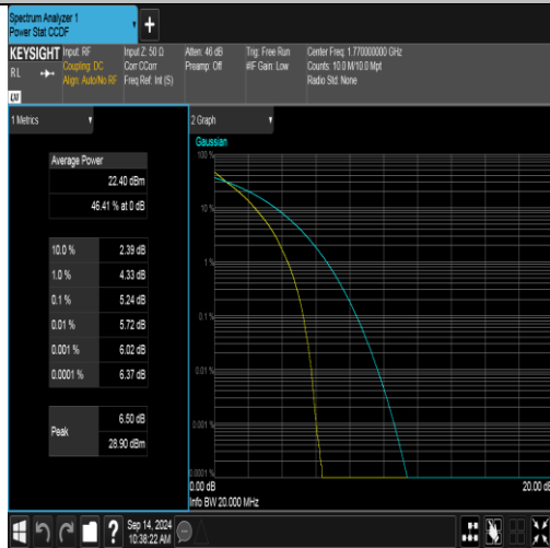
Band66-20MHz-QPSK-132572-100RB#0-PASS
