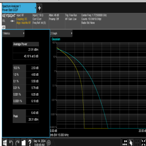
Band66-15MHz-QPSK-132597-75RB#0-PASS
