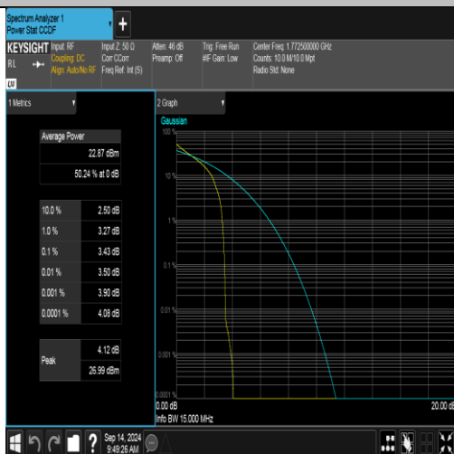
Band66-15MHz-QPSK-132597-1RB#0-PASS
