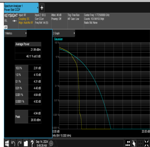
Band66-15MHz-16QAM-132597-1RB#0-PASS
