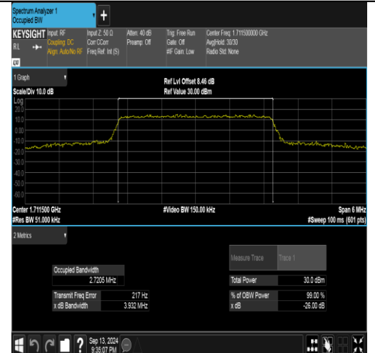
Band66-3MHz-16QAM-131987-15RB#0-PASS
