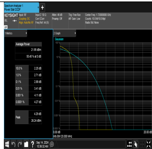
Band66-20MHz-16QAM-132072-1RB#0-PASS
