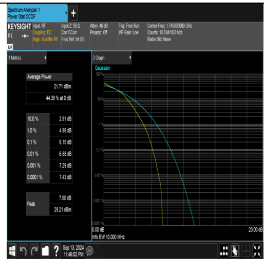
Band66-10MHz-16QAM-132322-50RB#0-PASS
