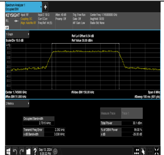
Band66-3MHz-16QAM-132322-15RB#0-PASS
