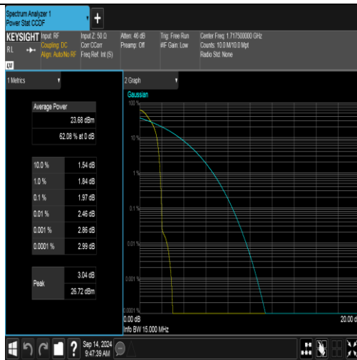
Band66-15MHz-QPSK-132047-1RB#0-PASS
