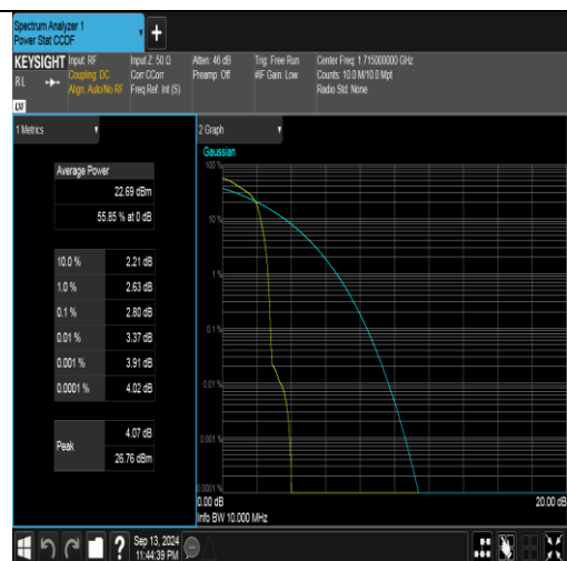
Band66-10MHz-16QAM-132022-1RB#0-PASS
