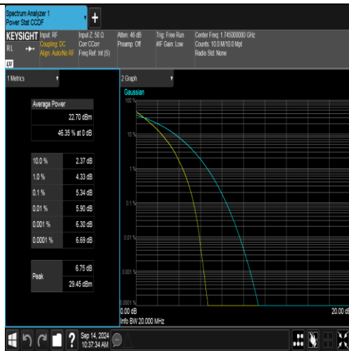
Band66-20MHz-QPSK-132322-100RB#0-PASS
