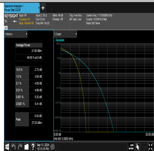
Band66-3MHz-16QAM-131987-15RB#0-PASS
