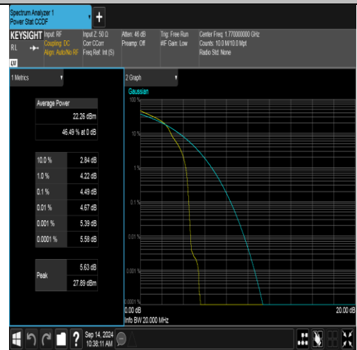
Band66-20MHz-16QAM-132572-1RB#0-PASS
