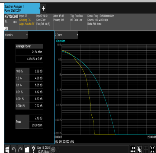
Band66-20MHz-16QAM-132322-1RB#0-PASS
