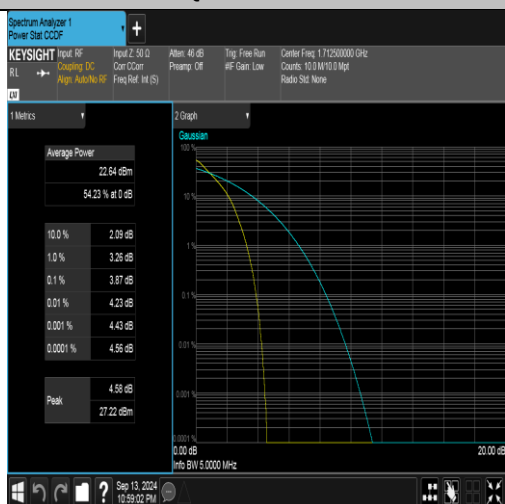
Band66-5MHz-QPSK-131997-25RB#0-PASS
