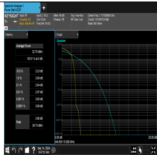
Band66-15MHz-16QAM-132047-1RB#0-PASS
