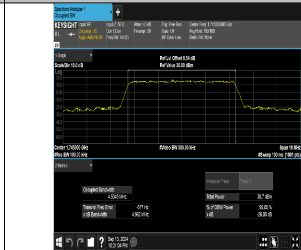
Band66-5MHz-16QAM-132322-25RB#0-PASS
