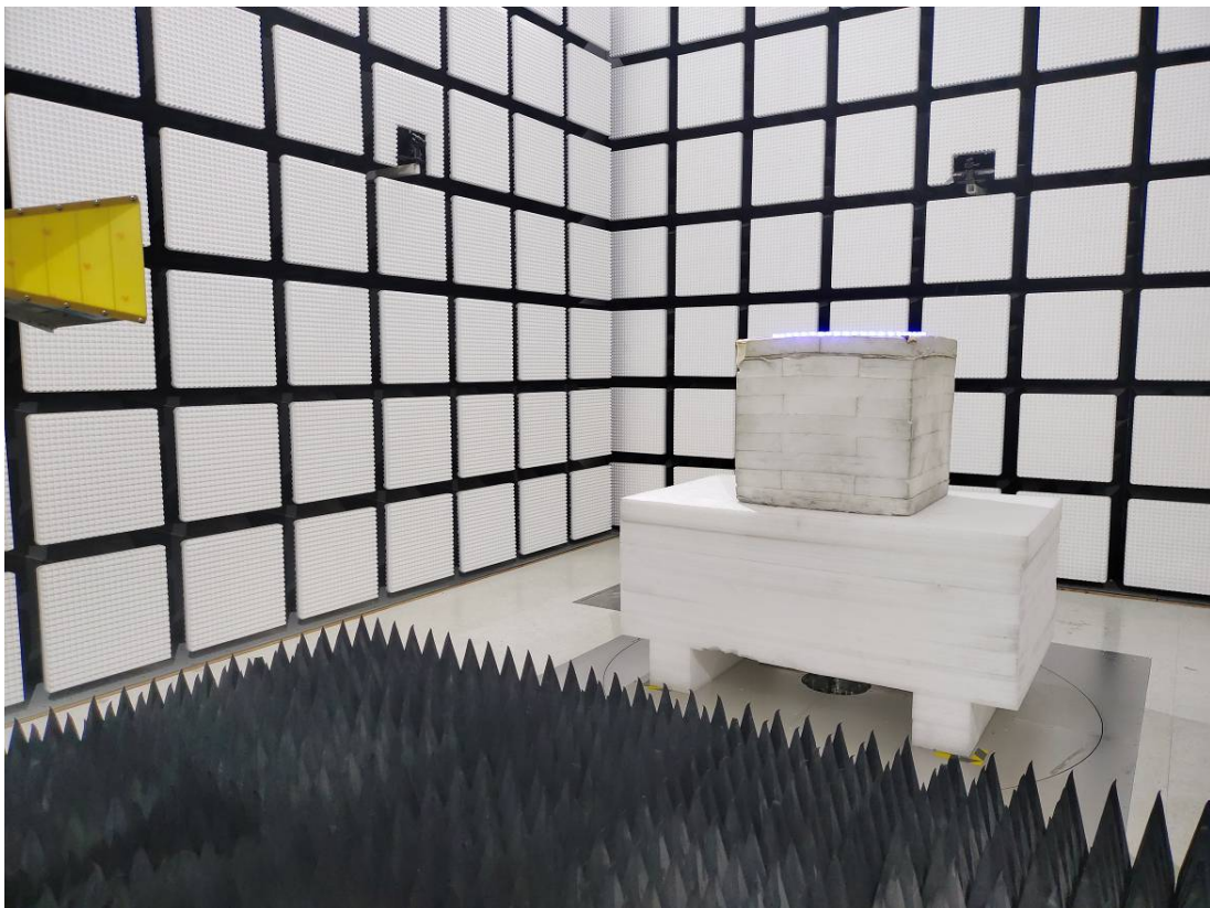
Radiated Emission Above 1GHz View(For model MLW7-1003-ICM)
