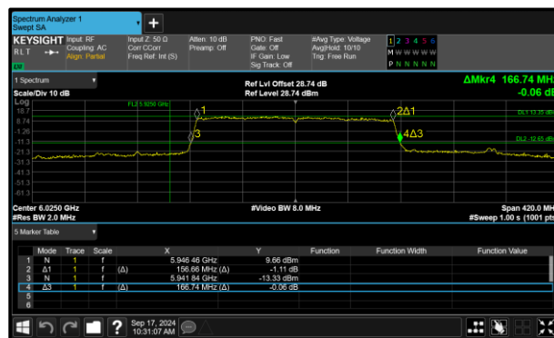
Figure 148 - 802.11ax HE160 SU SP Maximum 99% OBW
