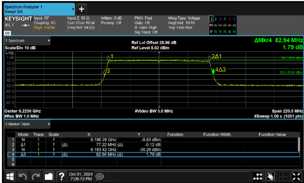
Figure 84 - 802.11ax HE80 SU VLP Maximum 26 dB EBW
