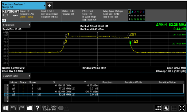
Figure 83 - 802.11ax HE80 SU VLP Minimum 26 dB EBW
