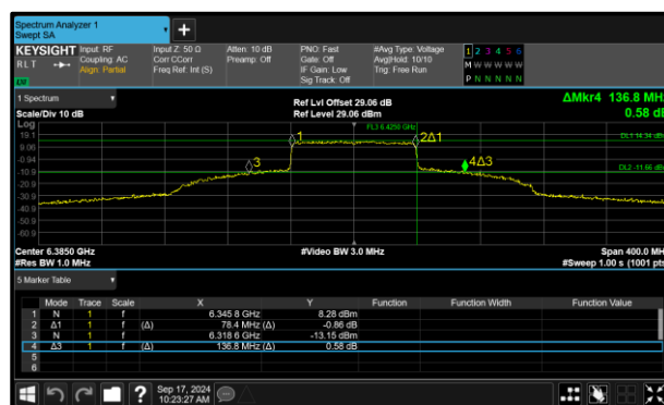
Figure 146 - 802.11ax HE80 SU SP Maximum 99% OBW
