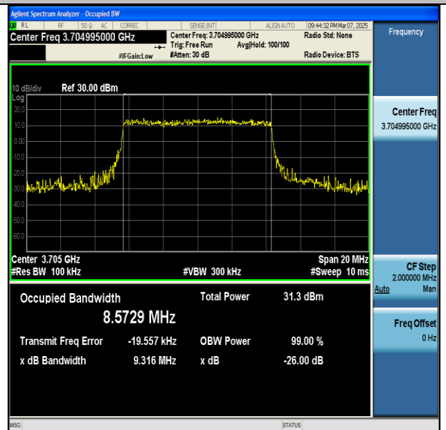
NTVN-n77(3700-3980)-PC2-30-10-L-CP-64QAM- Outer_Full-Ant1-PASS
