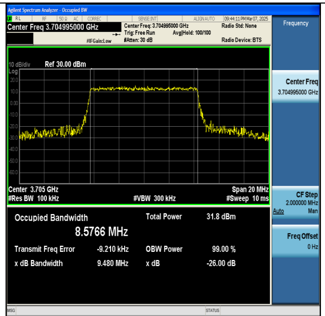
NTVN-n77(3700-3980)-PC2-30-10-L-CP-QPSK- Outer_Full-Ant1-PASS
