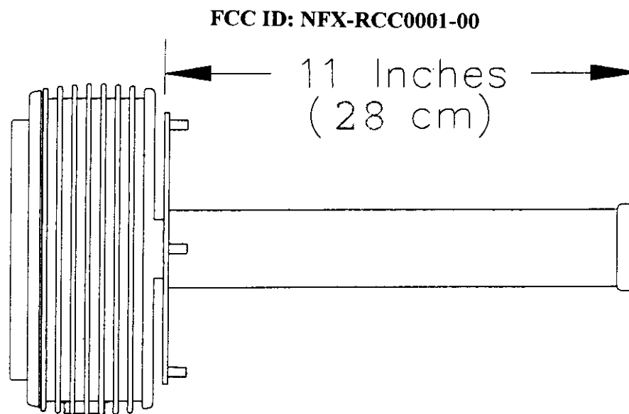
Figure 6-7. Helical Antenna
