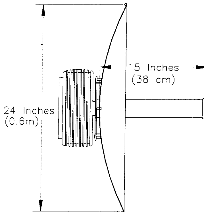
Figure 6-8. 0.6 Meter Dish Antenna
