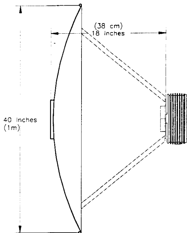
Figure 6-9. 1.0 Meter Dish Antenna
