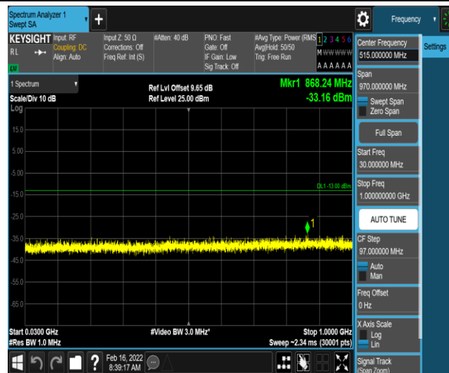
Band66-3MHz-QPSK-132322-1-0-Low-30-1000--33.16-PASS
