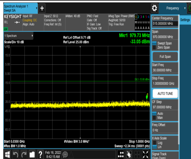
Band66-3MHz-QPSK-132657-1-0-High-30-1000--33.05-PASS
