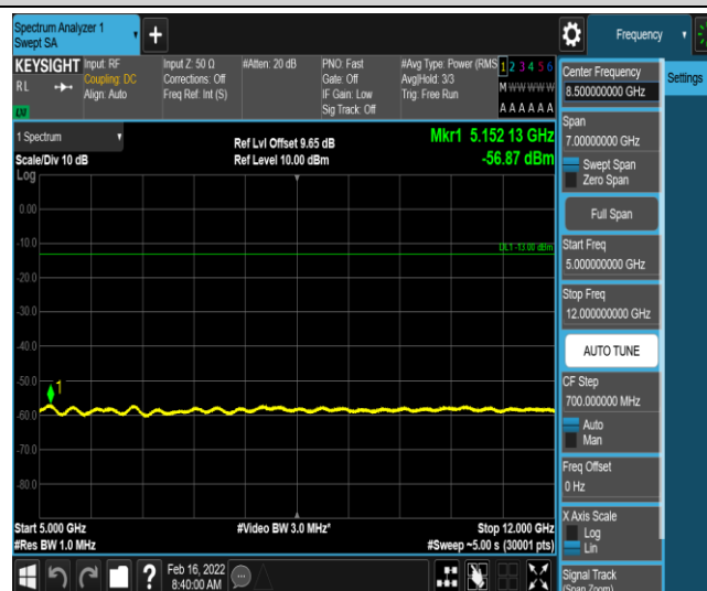
Band66-3MHz-QPSK-132322-1-0-Low-5000-12000--56.87-PASS
