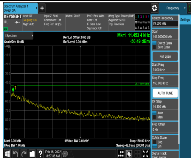
Band66-3MHz-16QAM-131987-1-0-Low-0.009-0.15--50.49-PASS
