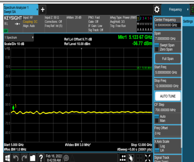
Band66-3MHz-QPSK-132657-1-0-High-5000-12000--56.77-PASS
