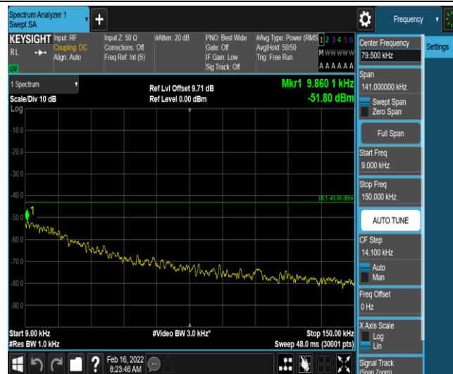
Band66-1.4MHz-16QAM-132665-1-0-High-0.009-0.15--51.8-PASS
