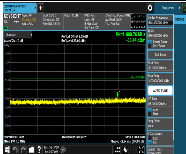
Band66-3MHz-16QAM-132322-1-0-Low-30-1000--33.47-PASS
