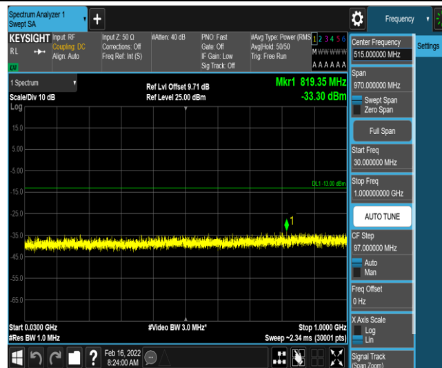
Band66-1.4MHz-16QAM-132665-1-0-High-30-1000--33.3-PASS
