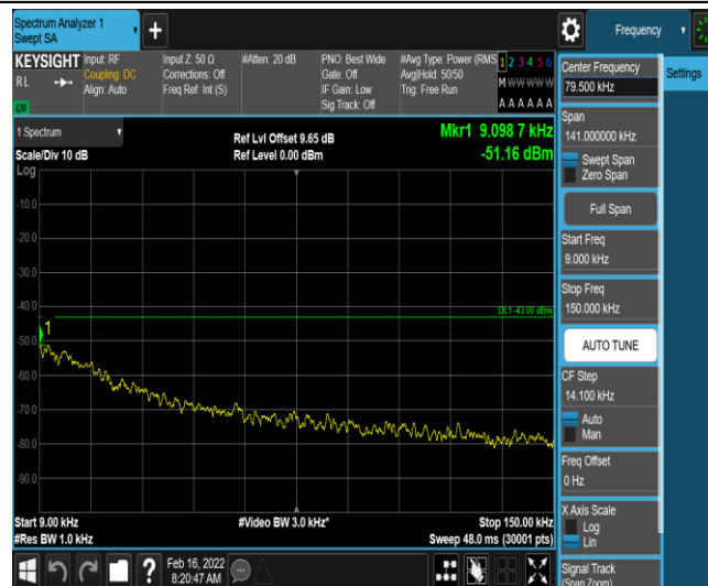
Band66-1.4MHz-16QAM-132322-1-0-Low-0.009-0.15--51.16-PASS
