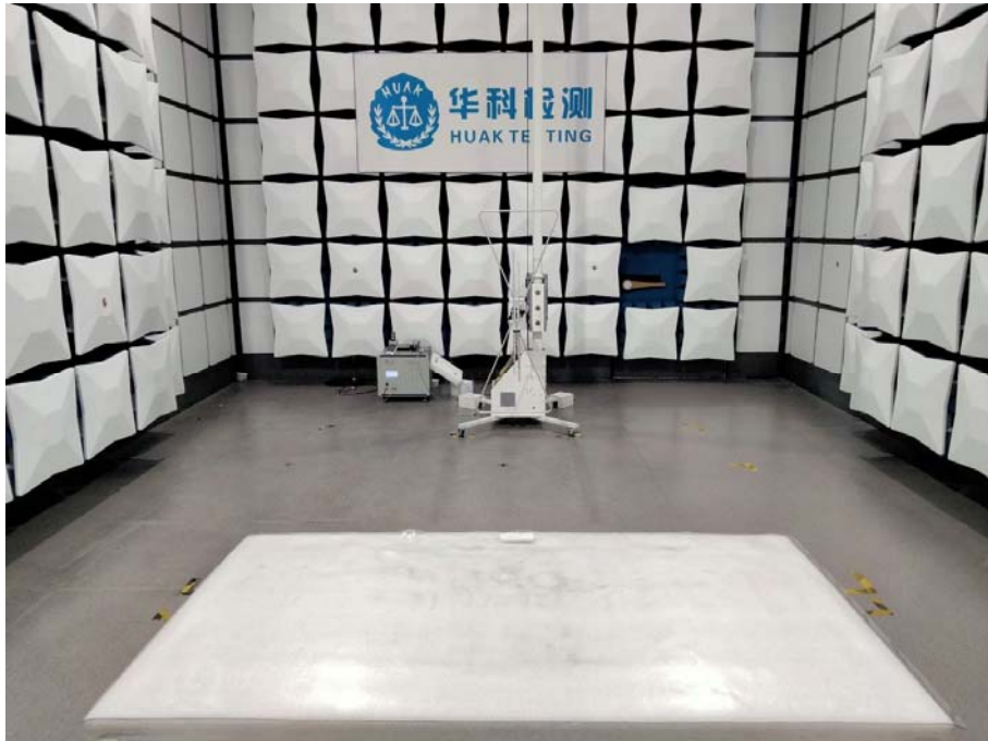
Model: FS400-A1 Radiated Emissions
