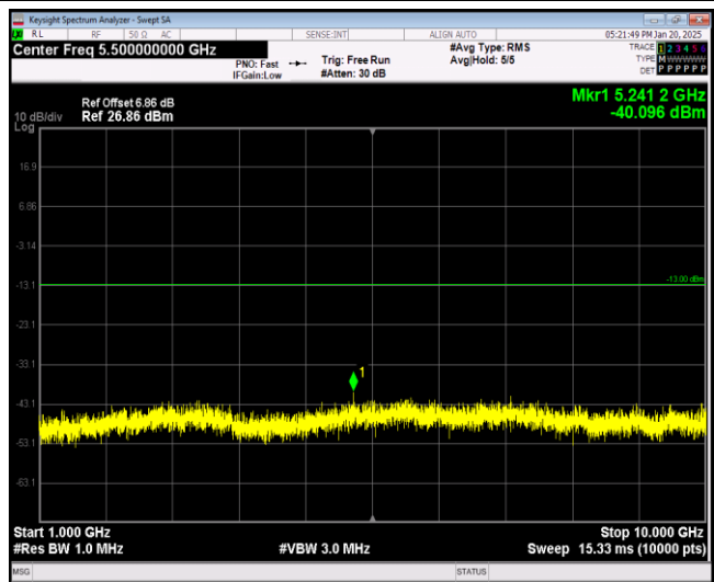
Band5-1.4MHz-QPSK-20525-1RB#0-Range2:1000~10000MHz
