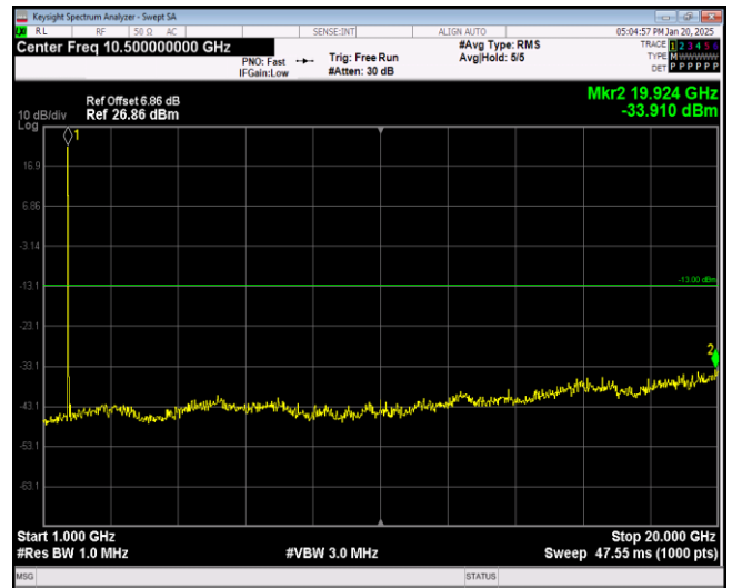
Band4-20MHz-16QAM-20175-1RB#0-Range2:1000~20000MHz
