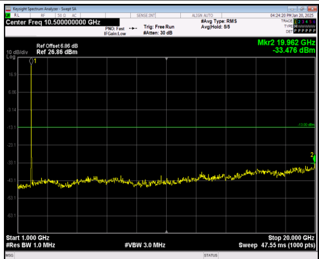
Band2-20MHz-64QAM-19100-1RB#0-Range2:1000~20000MHz
