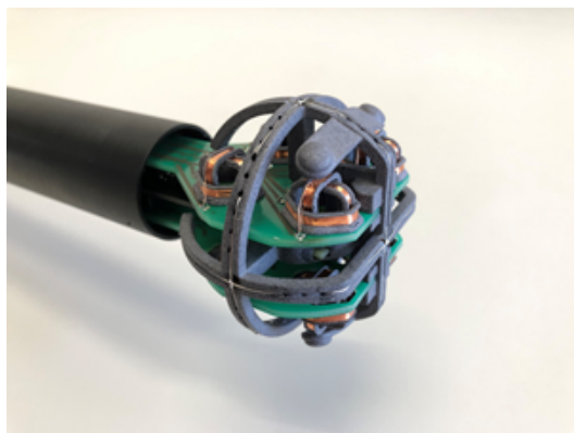
Test probe, without the casing
