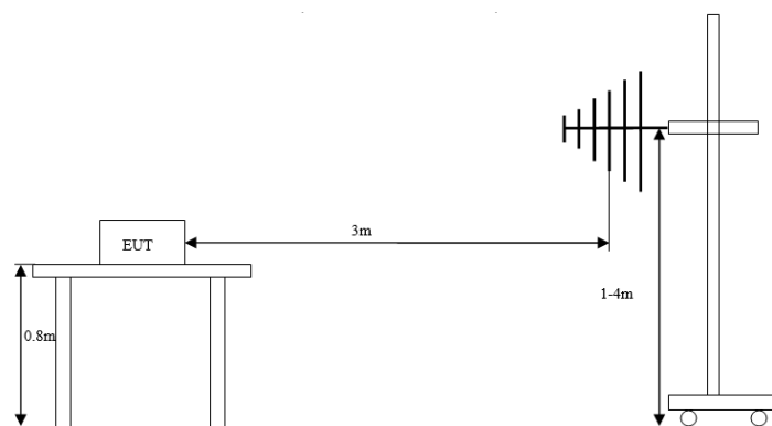
(Radiated emission)
