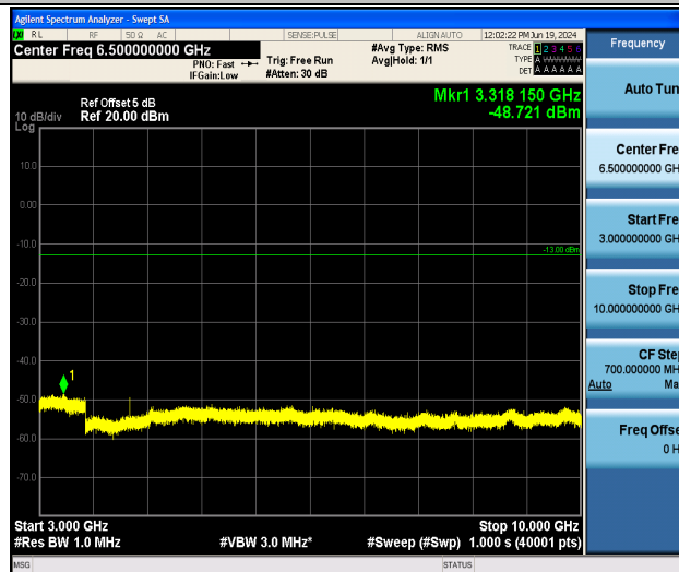
Band26_5MHz_16QAM_26915_1RB#0_3000~10000_3000~10000
