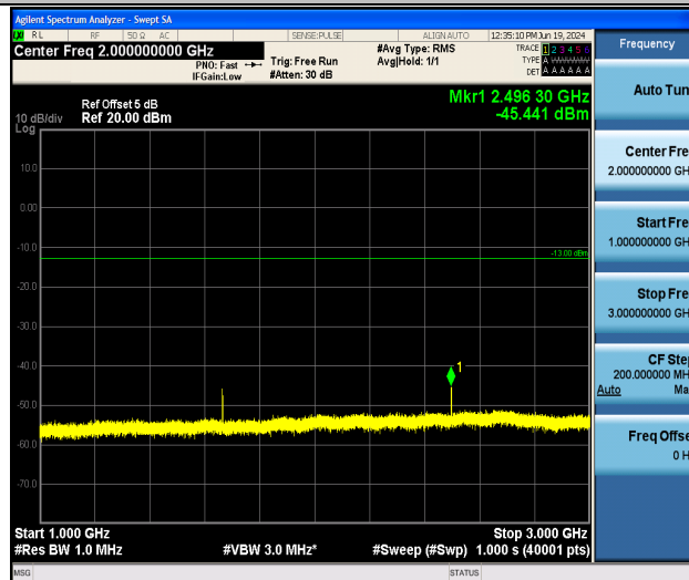
Band26_10MHz_QPSK_26915_1RB#0_1000~3000_1000~3000
