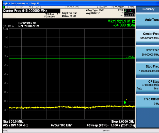
Band26_10MHz_16QAM_26990_1RB#0_30~1000_30~1000
