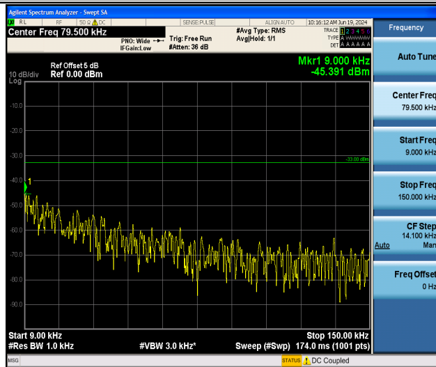
Band26_3MHz_16QAM_27025_1RB#0_0.009~0.15_0.009~0.15
