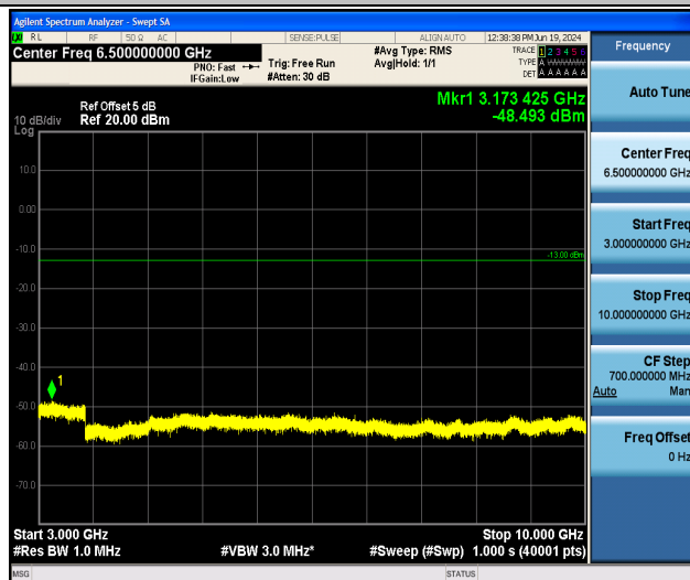
Band26_10MHz_16QAM_26990_1RB#0_3000~10000_3000~10000
