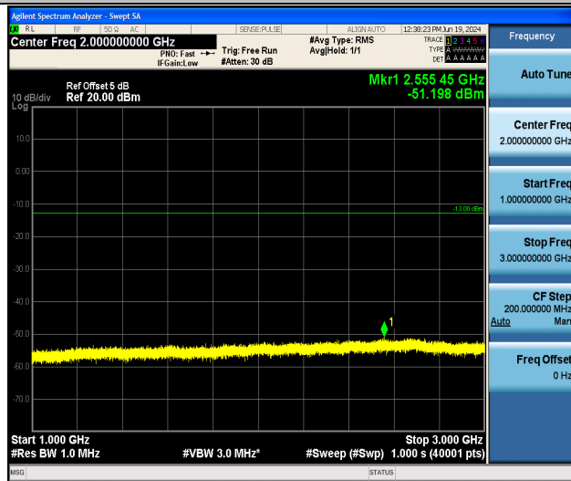
Band26_10MHz_16QAM_26990_1RB#0_1000~3000_1000~3000
