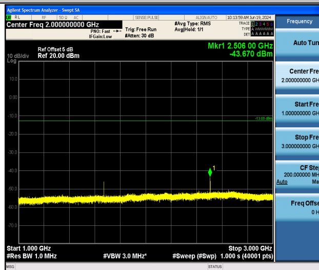
Band26_3MHz_QPSK_26915_1RB#0_1000~3000_1000~3000
