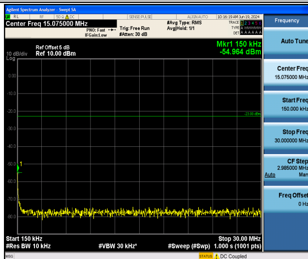
Band26_3MHz_16QAM_27025_1RB#0_0.15~30_0.15~30
