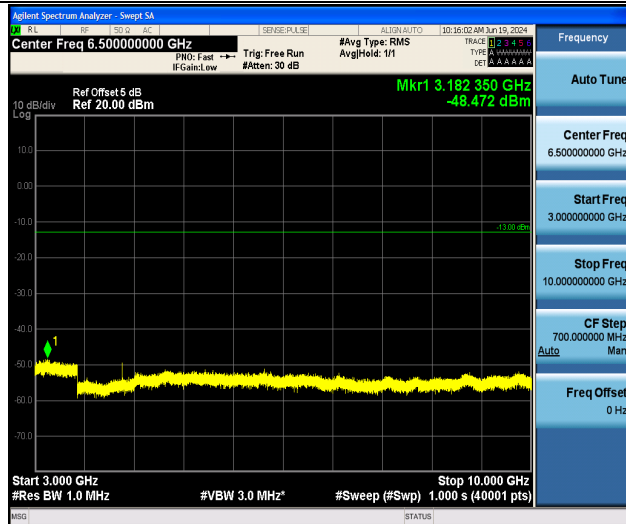
Band26_3MHz_QPSK_27025_1RB#0_3000~10000_3000~10000
