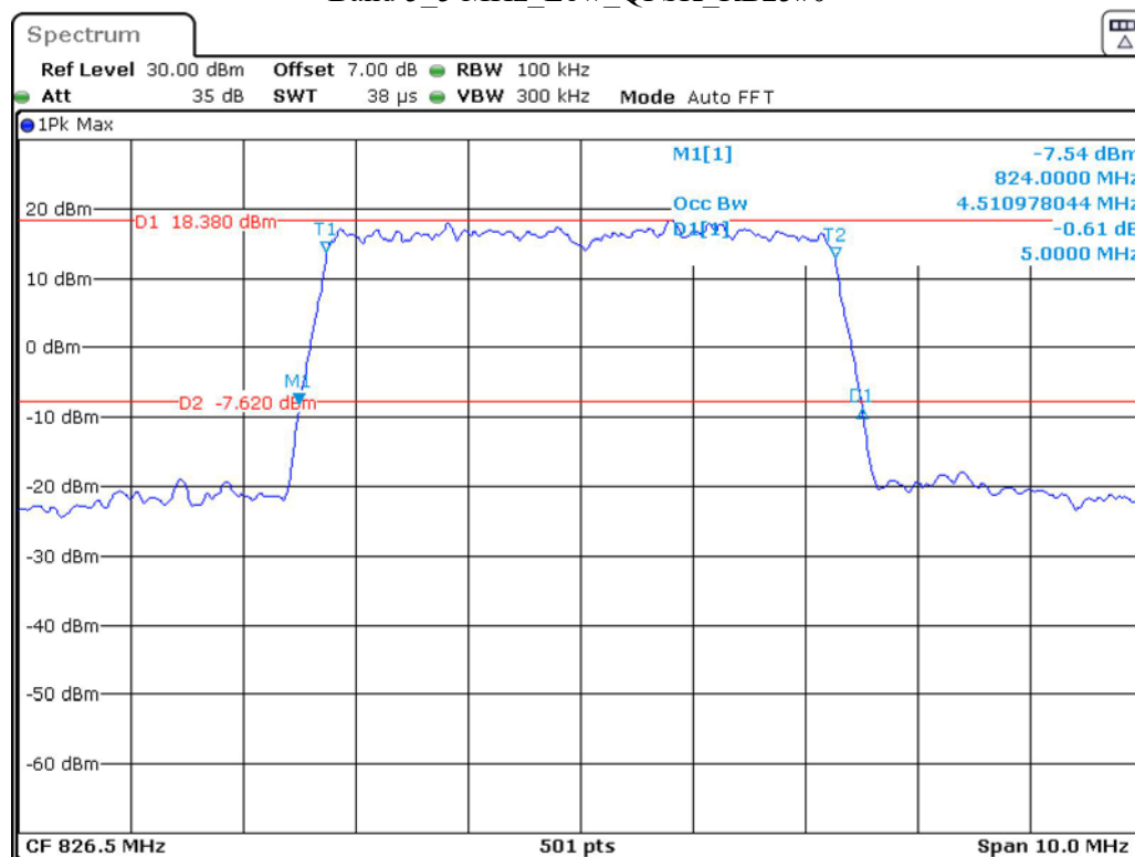
Band 5 5 MHz Low QPSK RB25#0
