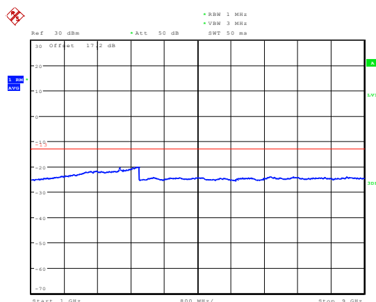
LTE Band 5 1.4MHz CH-Middle 1GHz ~9GHz
