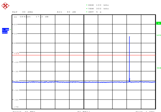
LTE Band 5 1.4MHz CH-Low 30MHz~1GHz
