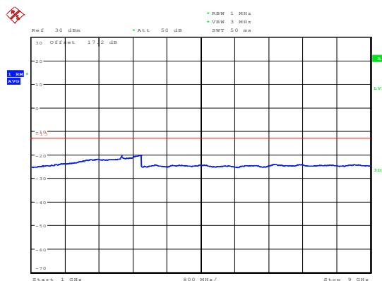
LTE Band 5 1.4MHz CH-Low 1GHz ~9GHz
