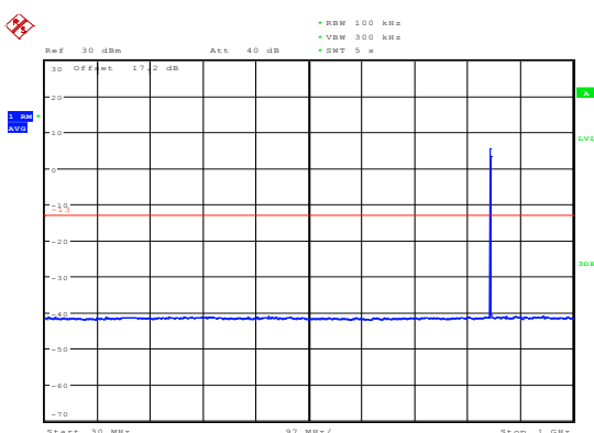
LTE Band 5 1.4MHz CH-High 30MHz~1GHz
