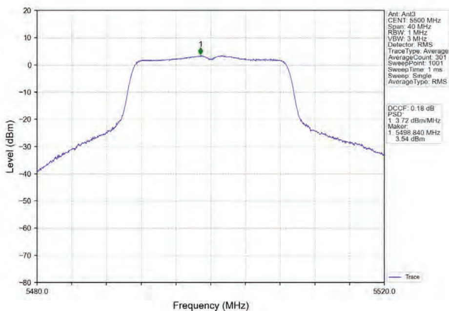
802.11ac(VHT20)_LCH_5500MHz_Ant3_NTNV
