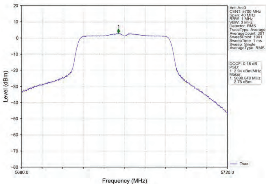
802.11ac(VHT20)_HCH_5700MHz_Ant3_NTNV
