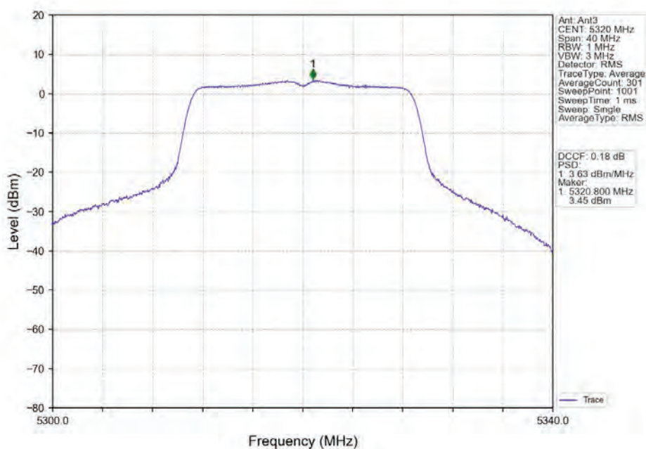
802.11ac(VHT20)_HCH_5320MHz_Ant3_NTNV
