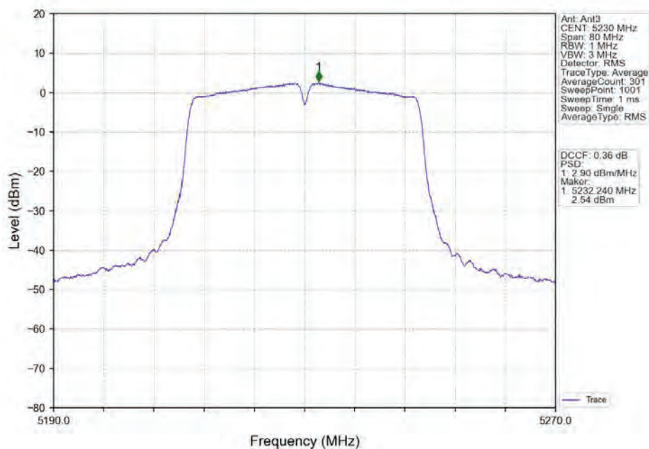
802.11ac(VHT40)_HCH_5230MHz_Ant3_NTNV
