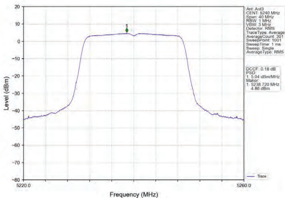
802.11ac(VHT20)_HCH_5240MHz_Ant3_NTNV
