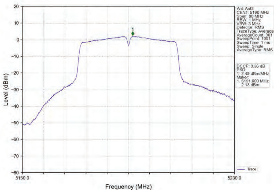
802.11ac(VHT40)_LCH_5190MHz_Ant3_NTNV
