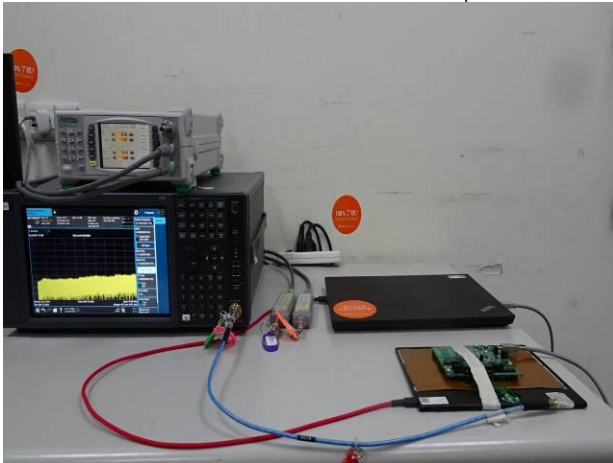
Part_15_209_EMR_Radiated_Setup
