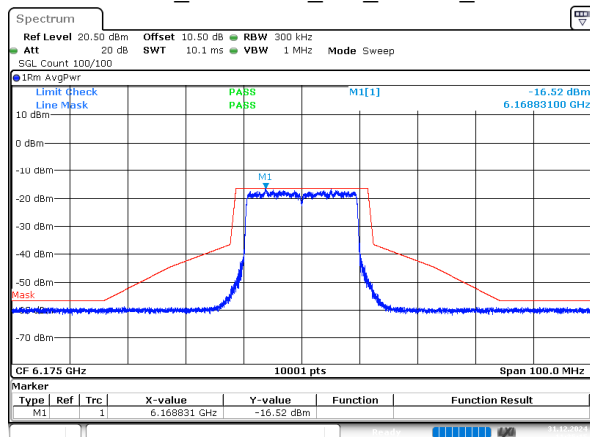
802.11ax20_6175MHz_RU_242/61_Chain 1
