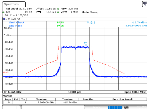
802.11ax20_5955MHz_RU_242/61_Chain 0
