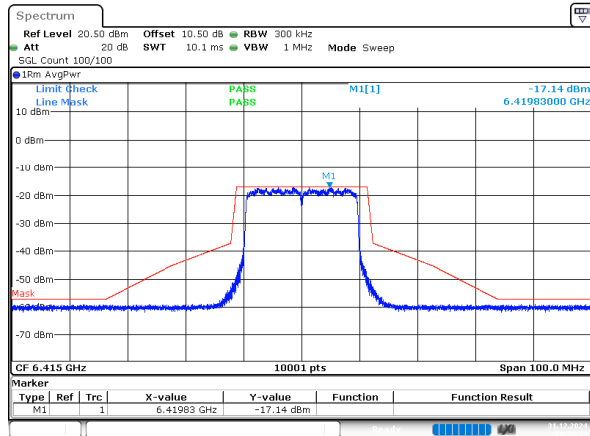
802.11ax20_6415MHz_RU_242/61_Chain 0
