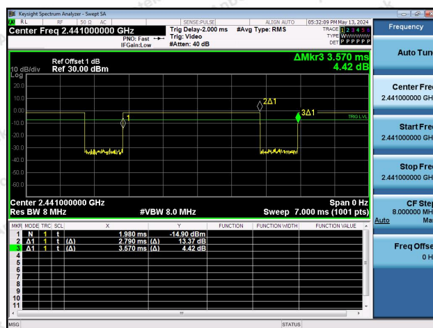
NTNV-DH5-Ant1-2441
