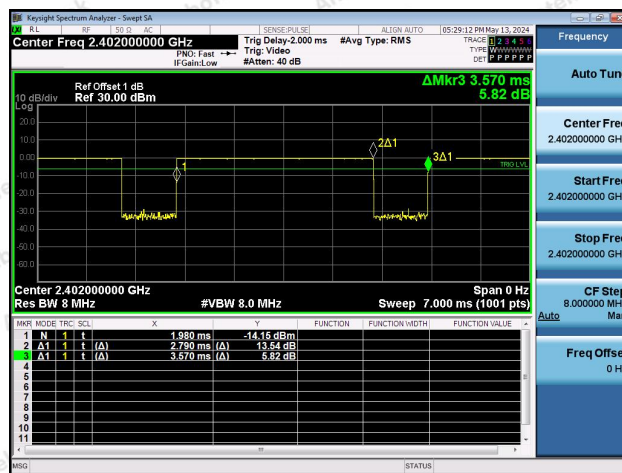
NTNV-DH5-Ant1-2402
