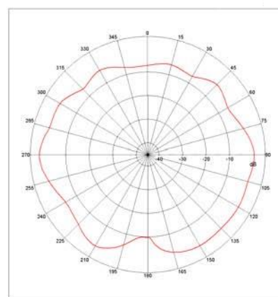
Far-field Power Distribution(H+V) on Y-Z Plane
