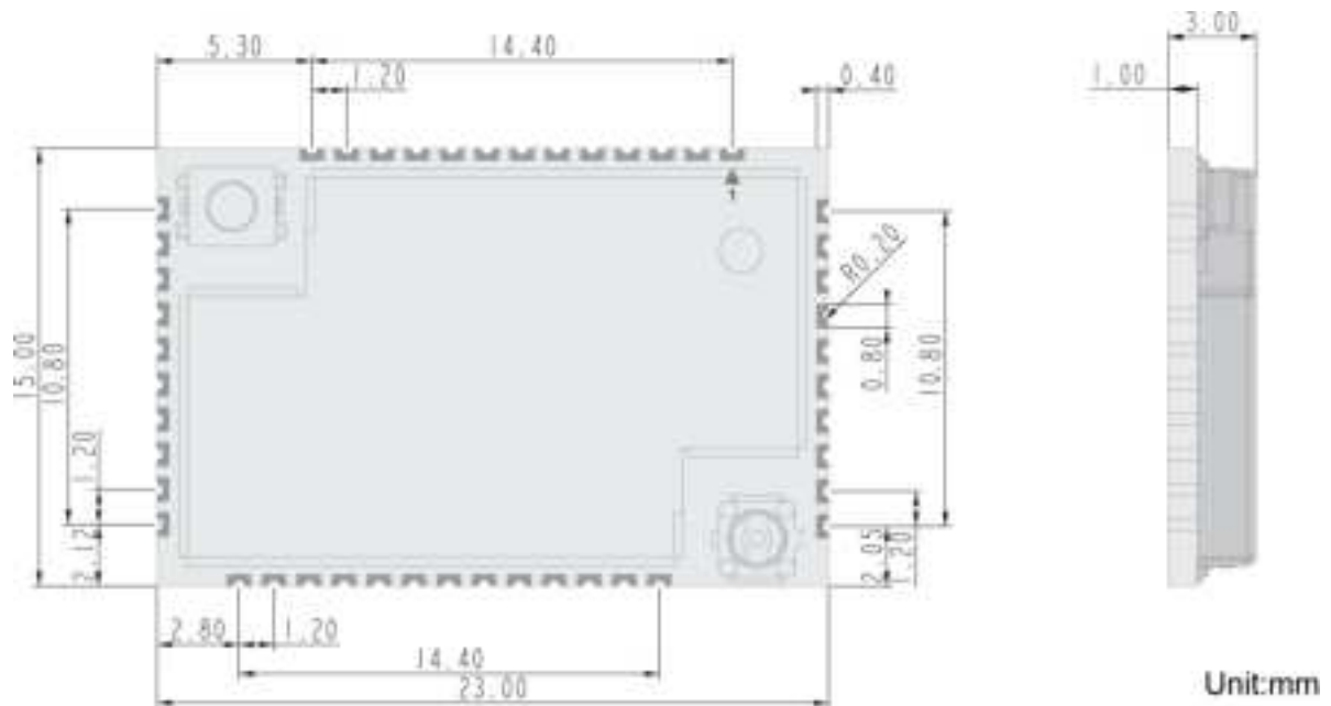
Figure 3: Mechanical Demensions
