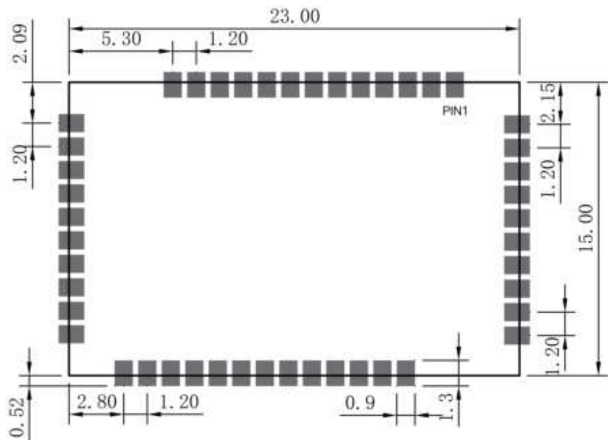
Figure 4: Recommended Footprint
