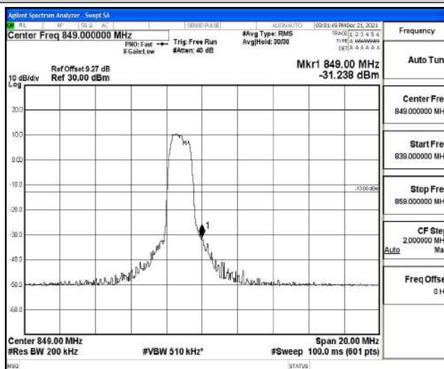
Band26-10MHz-16QAM-26990-6-0-High--31.24-PASS
