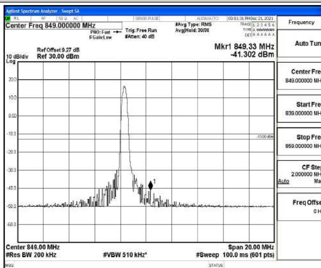
Band26-10MHz-16QAM-26990-1-0-High--41.30-PASS
