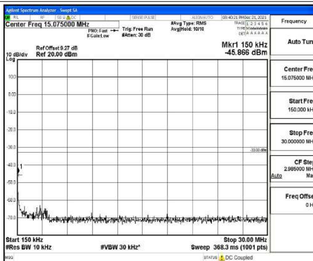
Band26-5MHz-16QAM-26865-1-0-Low-0.15-30--45.87-PASS
