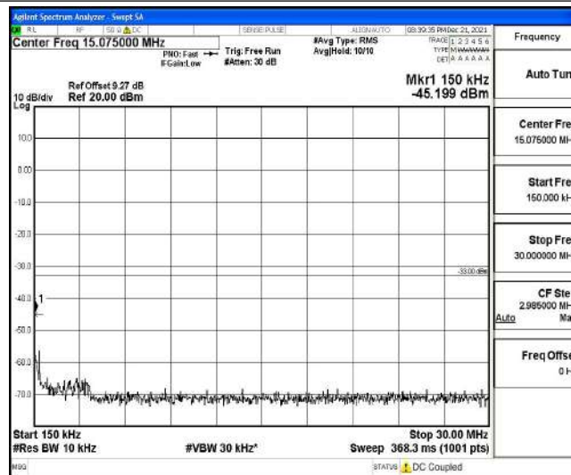
Band26-5MHz-QPSK-26865-1-0-Low-0.15-30--45.2-PASS
