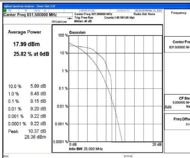
Band26-5MHz-QPSK-26865-1-0-Low-9.15-13-PASS
