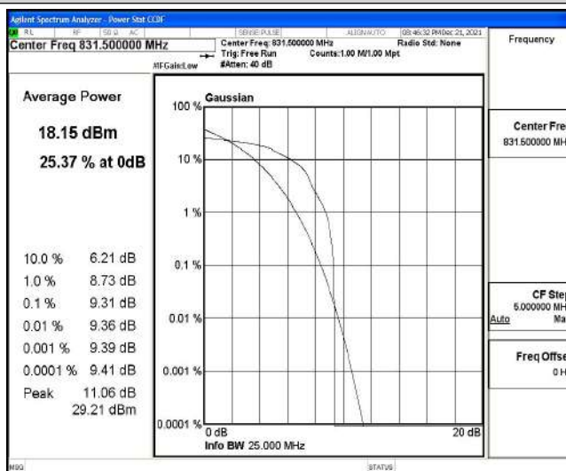
Band26-10MHz-16QAM-26865-1-0-Low-9.31-13-PASS
