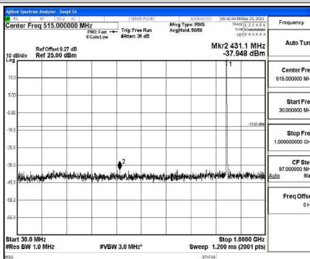
Band26-5MHz-16QAM-27015-1-0-High-30-1000--37.95-PASS
