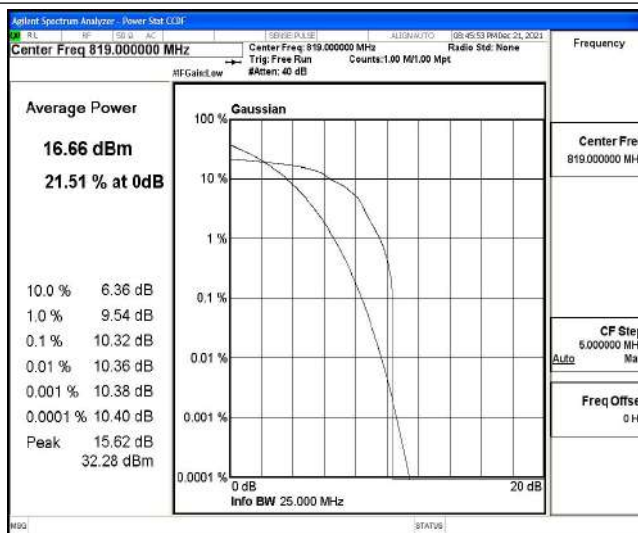
Band26-10MHz-16QAM-26740-1-0-Low-10.32-13-PASS
