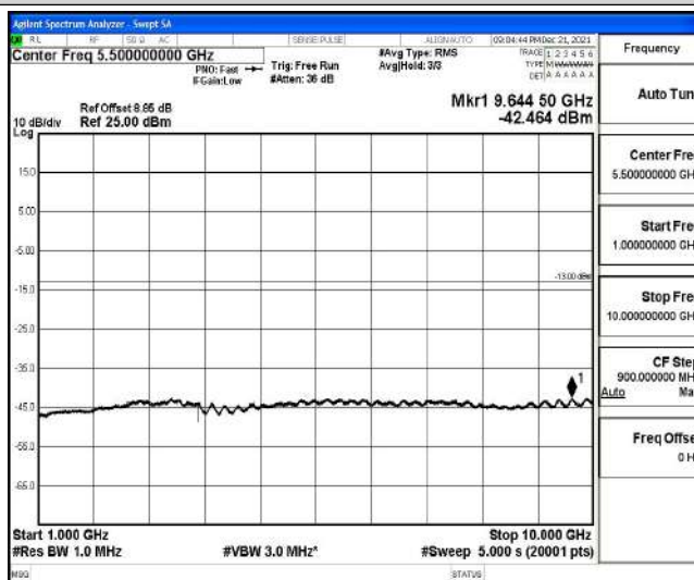
Band26-10MHz-QPSK-26740-1-0-Low-1000-10000--42.46-PASS
