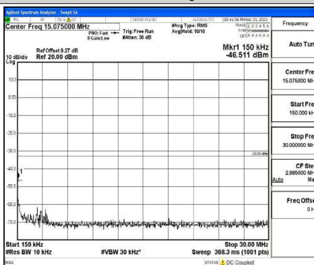
Band26-5MHz-16QAM-27015-1-0-High-0.15-30--46.51-PASS
