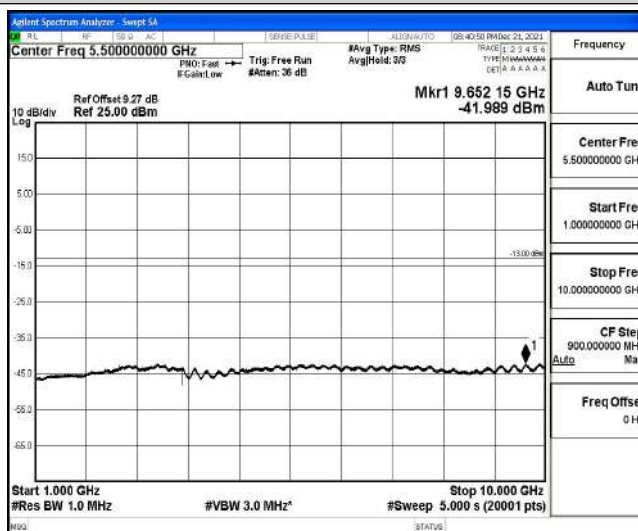
Band26-5MHz-16QAM-26865-1-0-Low-1000-10000--41.99-PASS
