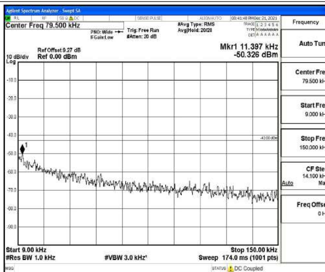
Band26-5MHz-16QAM-27015-1-0-High-0.009-0.15--50.33-PASS
