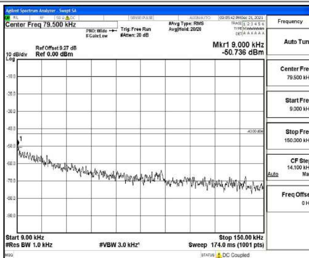
Band26-10MHz-QPSK-26865-1-0-Low-0.009-0.15--50.74-PASS
