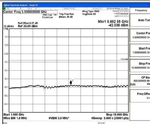
Band26-5MHz-QPSK-26865-1-0-Low-1000-10000--42.04-PASS
