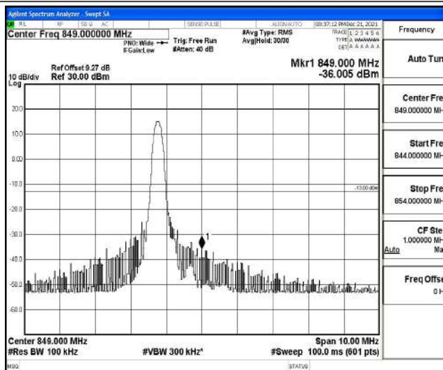
Band26-5MHz-QPSK-27015-1-0-High--36.01-PASS
