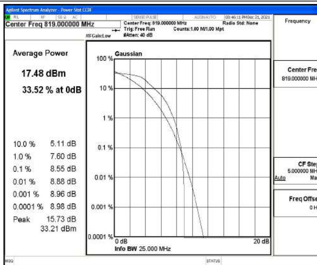
Band26-10MHz-16QAM-26740-6-0-Low-8.55-13-PASS
