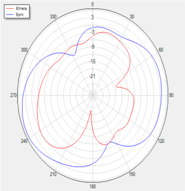
H Theta=90 freq=2480MHz
