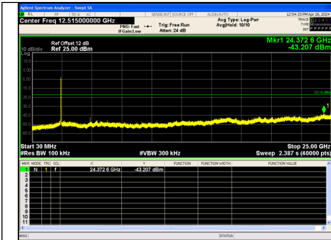
Spurious Emissions
