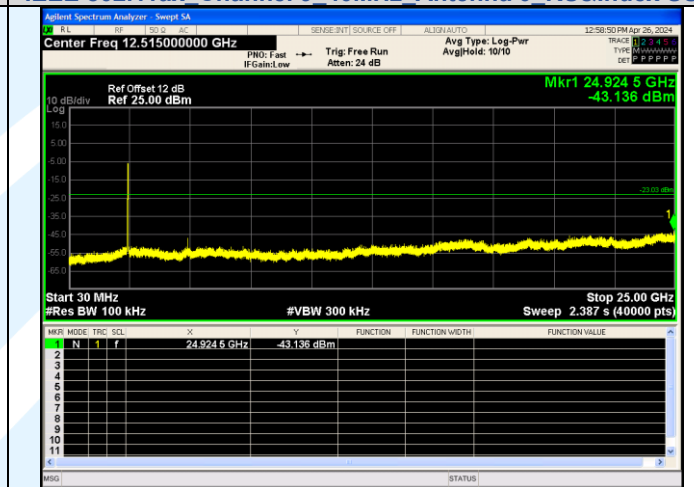
Spurious Emission
