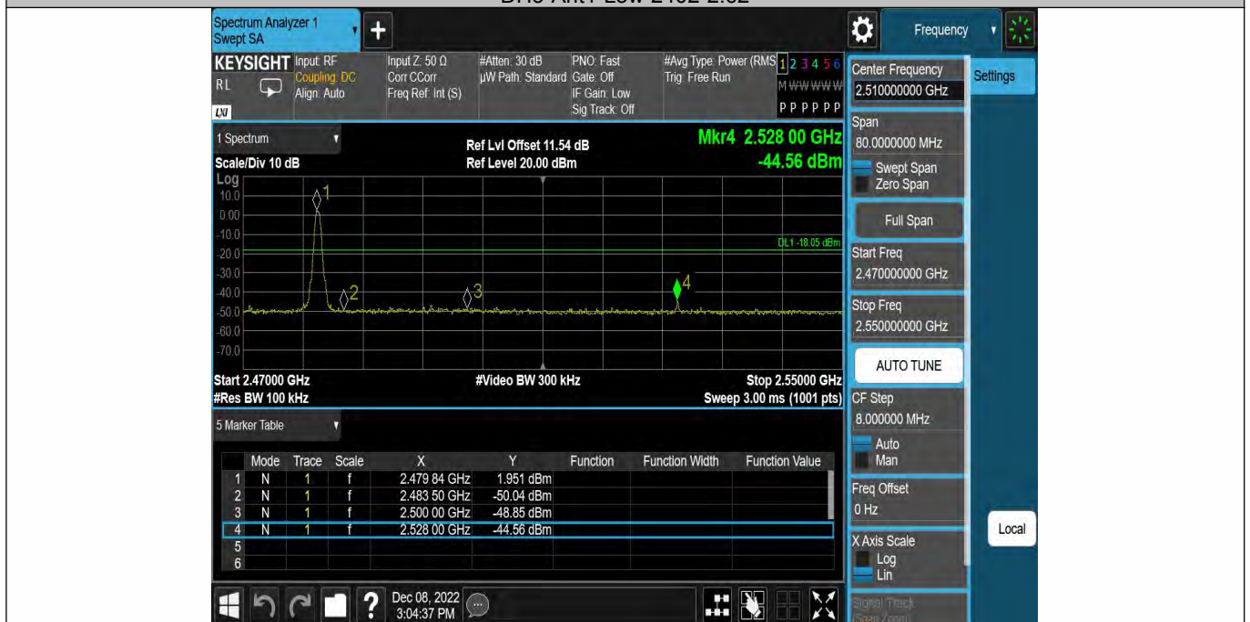
DH5-Ant1-High-2480-1.95
