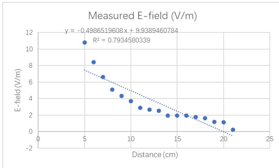
Figure 5 Linear model
