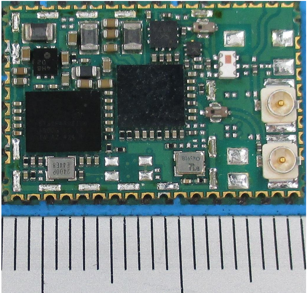
151496_03.jpg: EUT – Top View –Shielding removed (Odin-W260)
