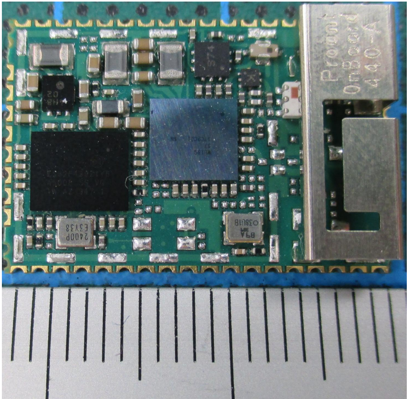
151496_05.jpg: EUT – Top View –Shielding removed (Odin-W262)
