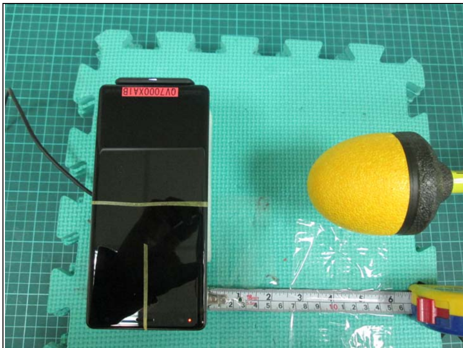
E-Field (Left) (Charging Mode)
