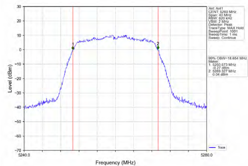
802.11ac(VHT20)_LCH_5260MHz_Ant1_NTNV
