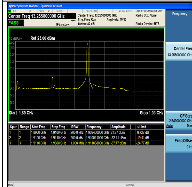
NTNV-n2-PC3-15-20-H-CP-QPSK-Edge_1RB_Right-PASS
