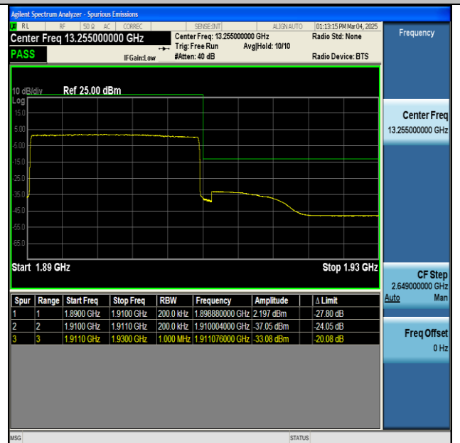
NTNV-n2-PC3-15-20-H-CP-QPSK-Outer_Full-PASS
