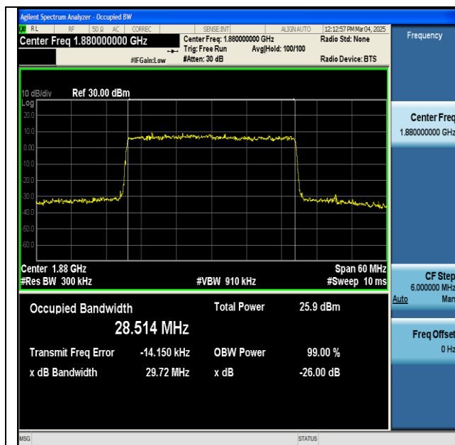
NTNV-n2-PC3-15-30-M-CP-256QAM-Outer_Full-Ant1-PASS
