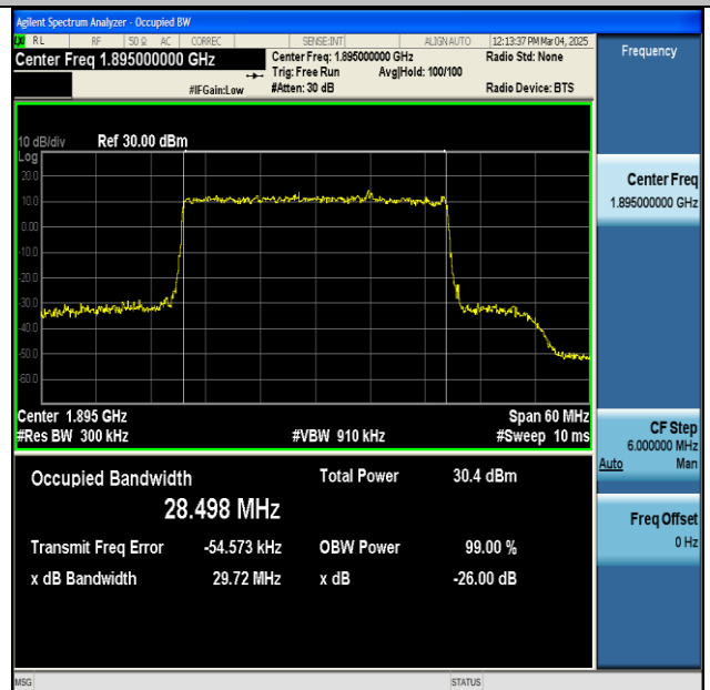
NTNV-n2-PC3-15-30-H-DFT-16QAM-Outer_Full-Ant1-PASS
