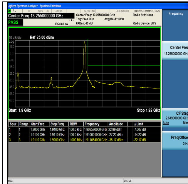
NTNV-n2-PC3-15-10-H-DFT-BPSK-Edge_1RB_Right-PASS
