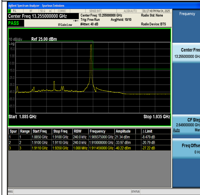
NTNV-n2-PC3-15-25-H-CP-QPSK-Edge_1RB_Right-PASS
