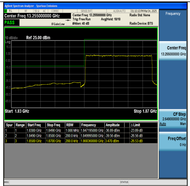
NTNV-n2-PC3-15-20-L-DFT-BPSK-Outer_Full-PASS
