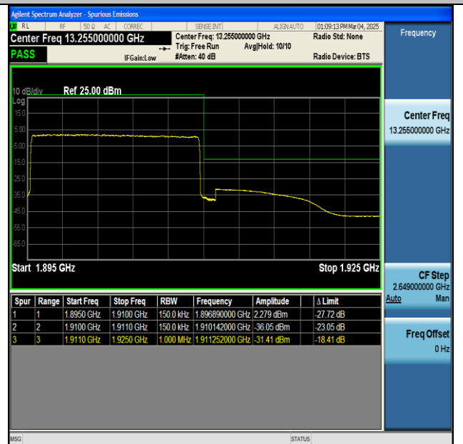
NTNV-n2-PC3-15-15-H-CP-QPSK-Outer_Full-PASS
