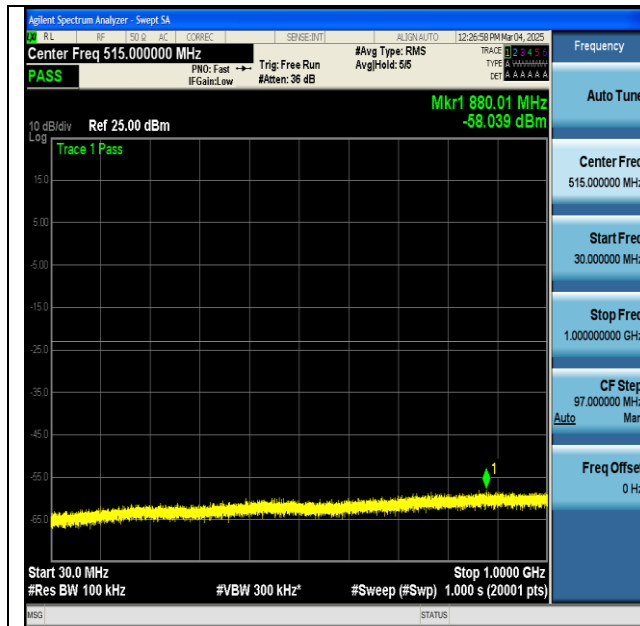
NTNV-n2-PC3-15-30-M-CP-QPSK-Edge_1RB_Left-30-1000-PASS
