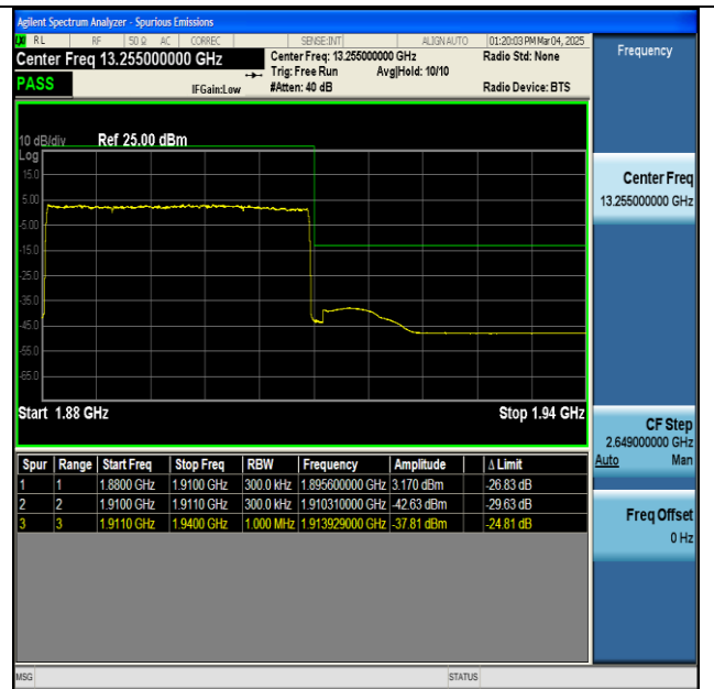
NTNV-n2-PC3-15-30-H-DFT-BPSK-Outer_Full-PASS
