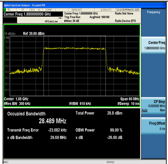
NTNV-n2-PC3-15-30-M-CP-64QAM-Outer_Full-Ant1-PASS
