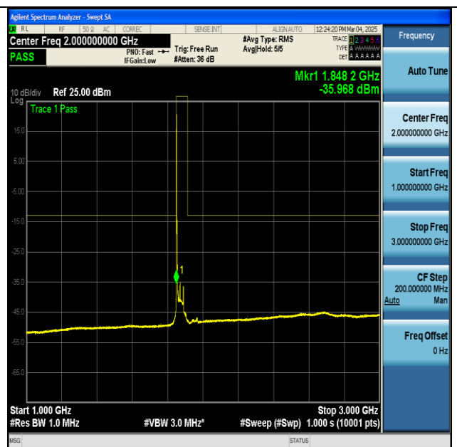
NTNV-n2-PC3-15-30-L-CP-QPSK-Edge_1RB_Left-1000-3000-PASS
