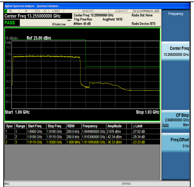
NTNV-n2-PC3-15-20-H-DFT-BPSK-Outer_Full-PASS
