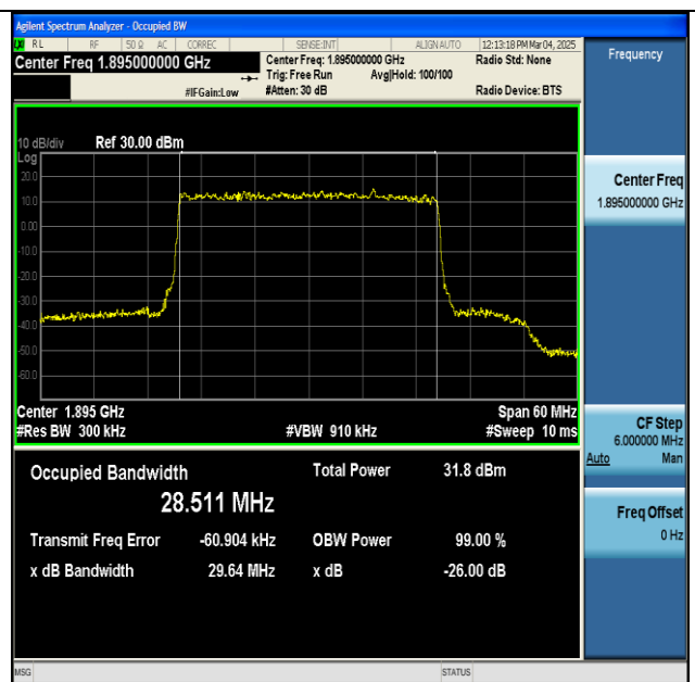
NTNV-n2-PC3-15-30-H-DFT-BPSK-Outer_Full-Ant1-PASS
