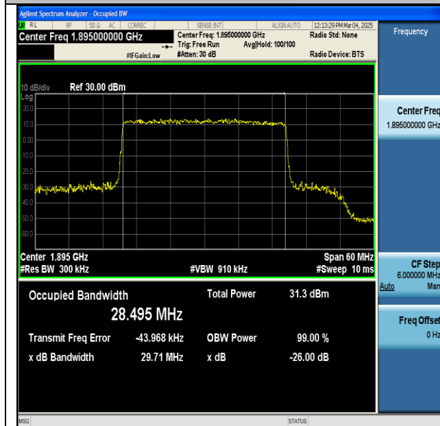
NTNV-n2-PC3-15-30-H-DFT-QPSK-Outer_Full-Ant1-PASS
