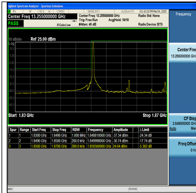
NTNV-n2-PC3-15-20-L-DFT-BPSK-Edge_1RB_Left-PASS
