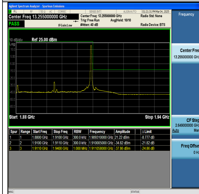
NTNV-n2-PC3-15-30-H-CP-QPSK-Edge_1RB_Right-PASS
