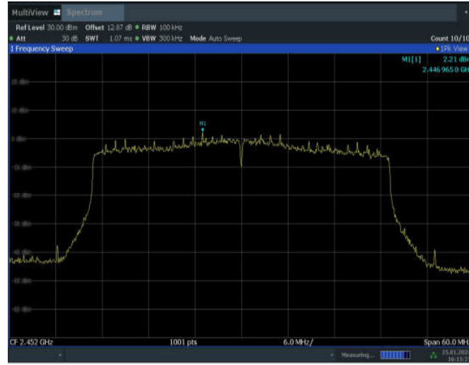
11AX40SISO_ANT5_2452_0~Reference
