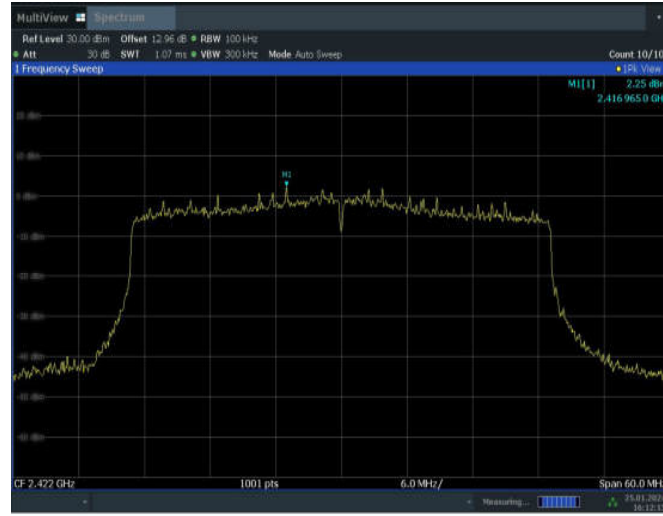
11AX40SISO_ANT5_2422_0~Reference
