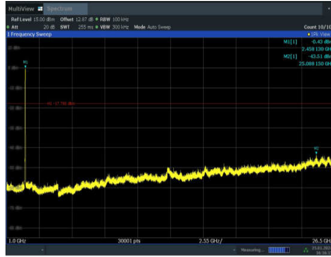
11AX40SISO_ANT5_2452_1000~26500
