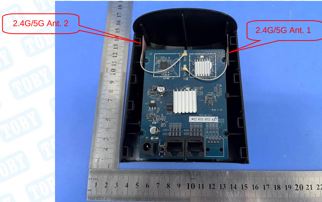
Photo 12 Appearance of PCB
