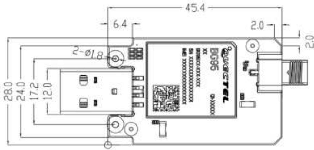
Figure 3.1: Topside view of QDM023-BG95-M1 communication module board
